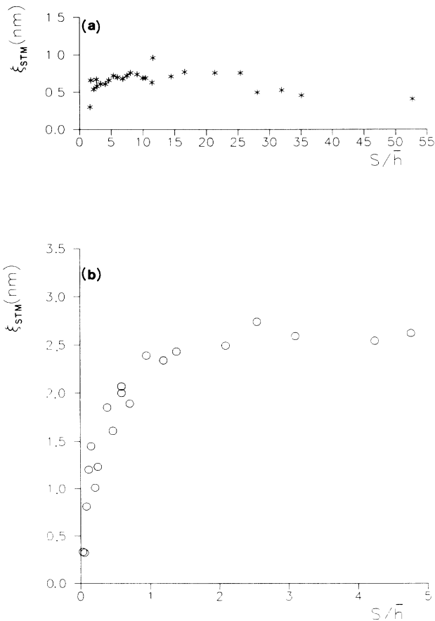
FIG. 6. \xi_{\text{STM}} vs S/\bar{h} plot for (a) \bar{h} = 30 nm and (b) \bar{h} = 850 nm.
