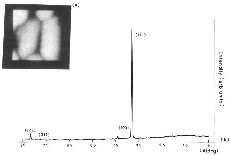
FIG. 3. (a) 70 \times 70 \text{ nm}^2 gray scale STM image (top view) of a gold deposit ( \bar{h} = 160 \text{ nm} ). (b) X-ray-diffraction pattern corresponding to a vapor gold film.
