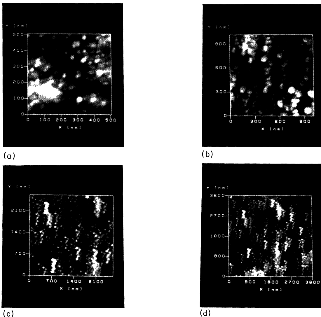
FIG. 4. Gray scale STM images (top view) of a gold deposit ( \bar{h} = 850 nm) at different magnifications.
