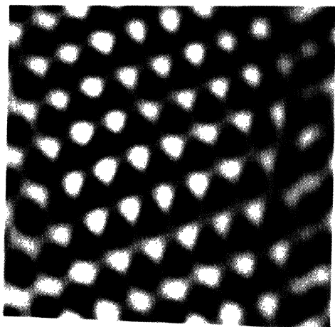
FIG. 1. 1.5 \times 1.5 \text{ nm}^2 top-view STM image of HOPG.
