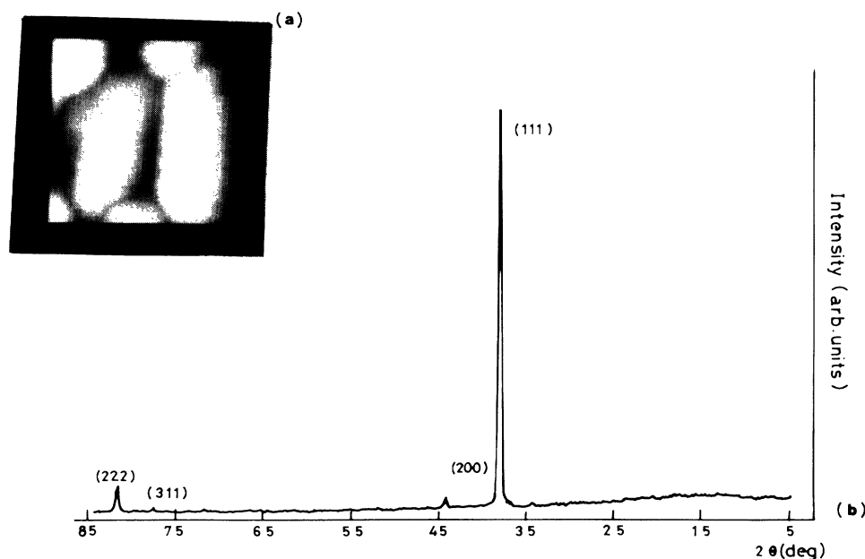
FIG. 3. (a) 70 \times 70 \text{ nm}^2 gray scale STM image (top view) of a gold deposit ( \bar{h} = 160 \text{ nm} ). (b) X-ray-diffraction pattern corresponding to a vapor gold film.
