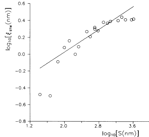
FIG. 11. \log_{10}\xi_{\text{STM}} vs S plot from data shown in Fig. 6(b).
