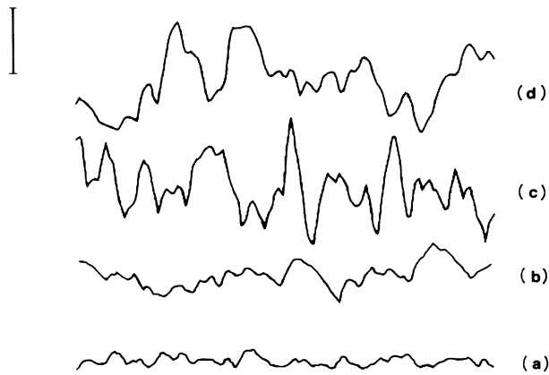
FIG. 5. Typical STM scans covering 974 nm for vapor-deposited gold films with different \bar{h} values. (a) \bar{h} = 30 nm, (b) \bar{h} = 160 nm, (c) \bar{h} = 500 , and (d) \bar{h} = 850 nm. The bar indicates 6 nm in the z direction.
