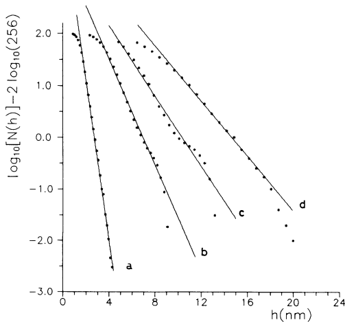
FIG. 10. \log_{10}N(h) vs h plots for S=1000 nm (a) \bar{h}=30 nm, (b) \bar{h}=160 nm, (c) \bar{h}=500 nm and (d) \bar{h}=850 nm.
