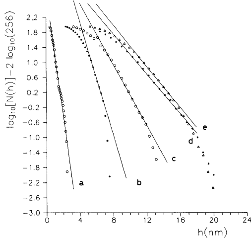
FIG. 9. \log_{10}N(h) vs h plots for \bar{h}=850 nm, (a) S=46.7 nm, (b) S=214 nm, (c) S=605 nm, (d) S=1000 nm and (e) S=3600 nm.
