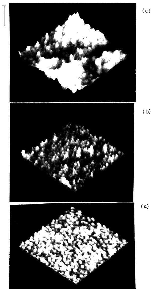
FIG. 2. 3D STM images of a vapor-deposited Au film. (a) 640 \times 640 \text{ nm}^2 , \bar{h} = 30 \text{ nm} ; (b) 600 \times 600 \text{ nm}^2 , \bar{h} = 160 \text{ nm} ; (c) 510 \times 510 \text{ nm}^2 , \bar{h} = 850 \text{ nm} . The bar indicates 18 nm in the z direction.
