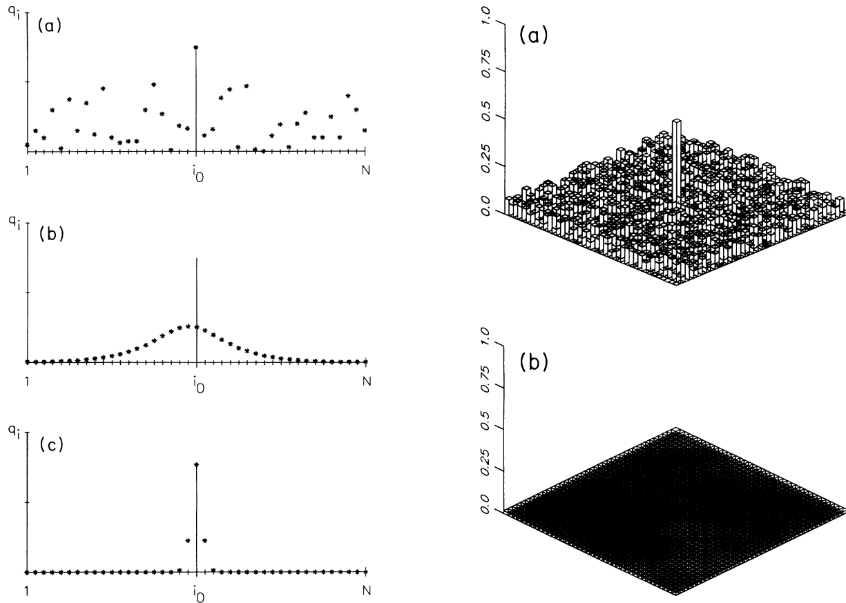
FIG. 7. Robust dynamical competition in one dimension: Neuron activity for (a) initial state, (b) final state of model I, and (c) final state of model II. N = 40 .
