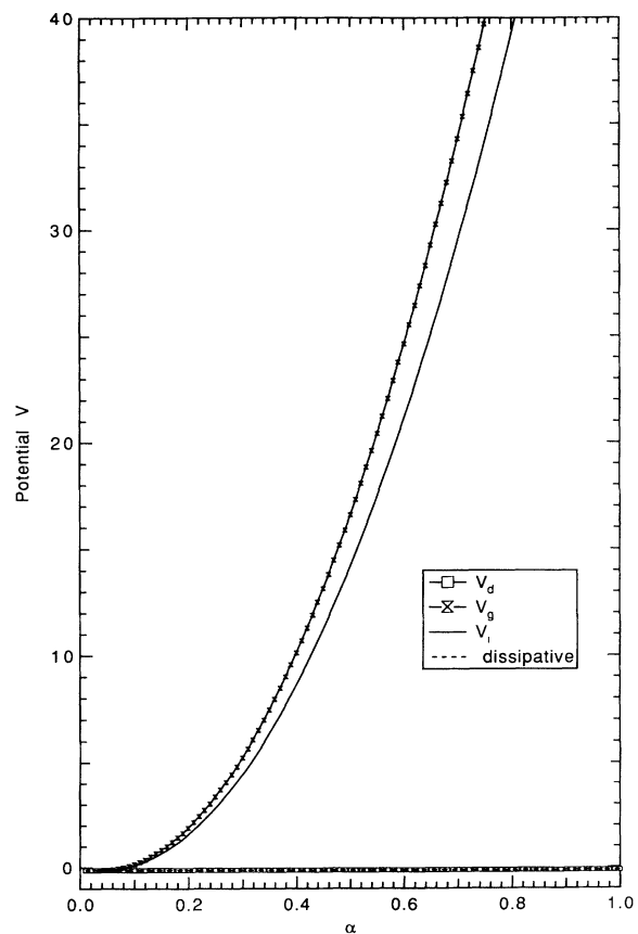
FIG. 5. Potential V of the ground states of model I in two dimensions as a function of the diffusive interaction: A comparison of simulations of the discrete model ( d ) with the Gaussian approximation ( g ), the lowest-order instanton ( i ), and the dissipative state.
