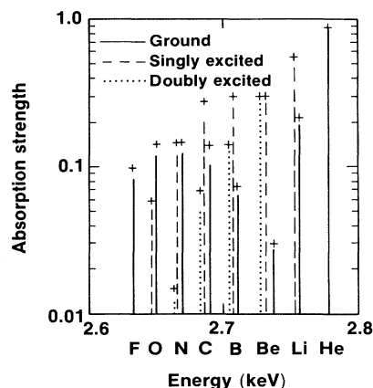
FIG. 4. This artificial spectrum is a plot of the average 1s-2p absorption strengths of the possible initial configurations of the heliumlike through fluorinelike ionization species of chlorine. Lines are positioned at the average transition energies. The crosses are values scaled from the heliumlike absorption strength given in Table I. Scaling with the square of the transition energy and with the vacancy fraction of the initial 2p subshell is seen to account for nearly all the changes in the average absorption strength.
