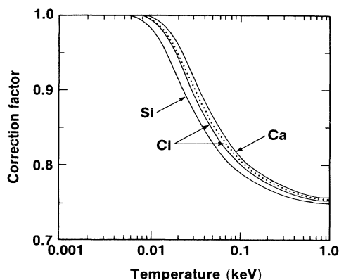
FIG. 3. The temperature-dependent absorption correction factor changes relatively little over the range of elements from silicon through calcium, as is shown here for the carbonlike species. Excitation energies used to calculate the solid curves were obtained using the screened hydrogenic approximation. The dashed line is the carbonlike chlorine curve from Fig. 2, which was derived from average excitation energies obtained using results from the atomic structure code (Ref. 10).
