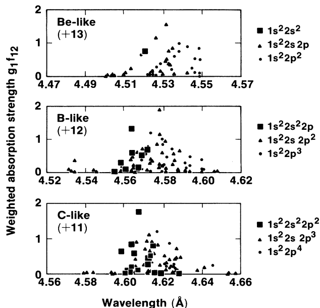
FIG. 1. Total statistical-weighted oscillator strengths for all significant (i.e., g_1 f_{12} > 0.01 ) transitions are plotted separately for the berylliumlike, boronlike, and carbonlike ionization species of chlorine. Transitions from the different initial configurations are distinguished. The line arrays from individual configurations are wider than the differences among the average transition energies for each configuration, but the total absorption bands for each species are separate enough to be distinct.
