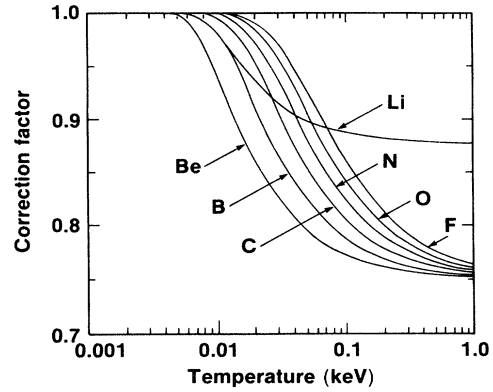
FIG. 2. The correction factor given by Eq. (6) is plotted for the relevant ionization species of chlorine. The total 1s - 2p absorption cross section for a particular species is obtained from the total cross section of the ground configuration alone by applying the appropriate factor.
