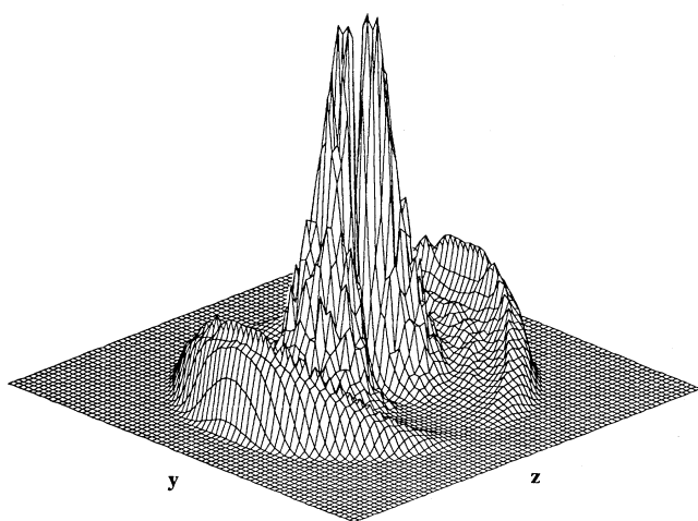
FIG. 2. A theoretical calculation of the probability density of the wave packet of Fig. 1 during the fractional revival. The y - z projection shows two sub-wave-packets, one at each extreme of the motion. The two sub-wave-packets oscillate at the classical orbital period.
