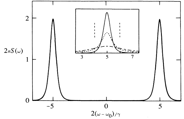
FIG. 1. (a) The spontaneous-emission spectrum 2\pi S(\omega) for \kappa \ll \gamma/2 and 2g/\gamma = 5 . The inset compares the spectral sidebands in free-space resonance fluorescence (Ref. 6), ---, the spontaneous-emission spectrum 2\pi S(\omega) , ···, and the fluorescent spectrum 2\pi T(\omega) , —. The vertical dashed lines show the full free-space radiative width \gamma .
