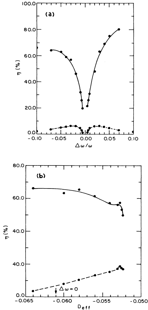
FIG. 1. The untapered (dashed line) and corresponding optimal tapered (solid line) efficiencies are plotted as functions of detuning parameters in the low-current limit. (a) The choice of v_\phi=1 corresponds to the CARM operating in vacuum. Other parameters used in the simulations are \omega_p=0.05 , \gamma_0=2.37 , and \theta_{p0}=0.53 . Upward tapering was used for the high-frequency branch with \Delta\omega > 0 , and downward tapering for the low-frequency branch with \Delta\omega < 0 . (b) A similar plot for \omega_p=0.005 and v_\phi=1.03 , corresponding to the CARM operating in a waveguide mode for the negative D_{\text{eff}} branch.
