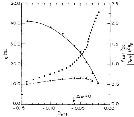
FIG. 2. The untapered efficiency (dashed line), corresponding optimal tapered efficiency (solid line) and ratio A_{\text{sat}} p_{z0} / |D_{\text{eff}}| k^2 \theta_p as functions of D_{\text{eff}} for v_\phi=1.03 , \omega_p=0.3 , \gamma_0=2.37 , and \theta_{p0}=0.53 .
