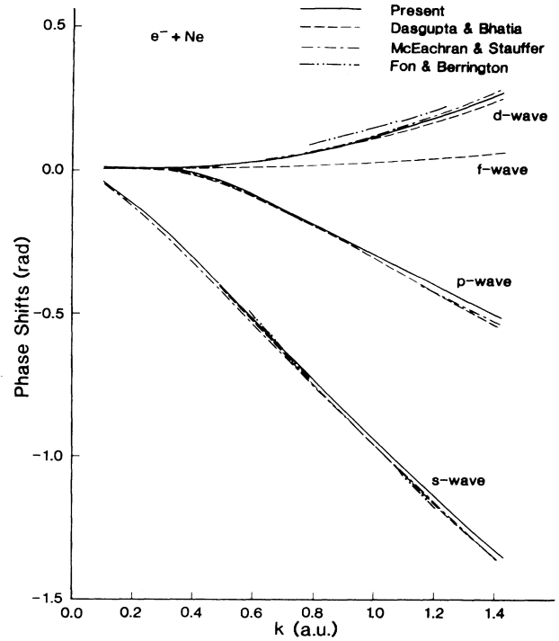
FIG. 1. s -, p -, d -, and f -wave phase shifts (mod \pi ) for the elastic scattering of electrons from neon atoms. —, MCSCF (present); ---, Dasgupta and Bhatia (Ref. 3); - · - · - ·, McEachran and Stauffer (Ref. 4); · · · · ·, Fon and Berrington (Ref. 5).
