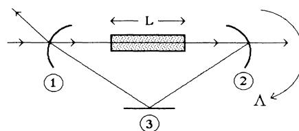
FIG. 3. Schematic representation of the ring cavity with spherical mirrors.
