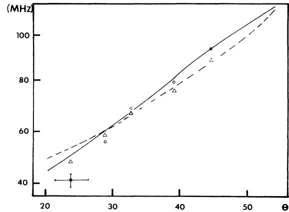
FIG. 19. Frequencies of oscillation ( \nu_+, \nu_- ) associated with the output-intensity boundaries of instability ( X_+, X_- ) in Fig. 13(a), for C=106\pm 5 , \Delta=-2.2\pm 0.2 , \kappa'=0.32 , and \gamma=1.6 as a function of cavity detuning \Theta in the out-of-confocal geometry b . Triangles are taken at the low-intensity boundary ( X_- ), circles are taken at the high-intensity boundary ( X_+ ). From the model of Lugiato et al. (Ref. 22) the dashed line shows the frequency ( \nu_- ) at the low-intensity boundary ( X_- ) while the continuous line is the frequency ( \nu_+ ) at the high-intensity boundary ( X_+ ). Systematic uncertainties in the detunings are \pm 10\% .
