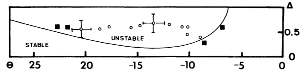
FIG. 16. Domain of instability in the detuning space for C=95\pm 5 ; open circles indicate instability; closed squares imply stability; above the continuous line is the theoretically unstable region. The confocal standing-wave resonator a is used with \kappa'=0.4 and \gamma=1.6 . The systematic uncertainties in the detunings are \pm 10\% .
