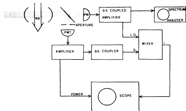
FIG. 14. Experimental arrangement for measurement of the transverse profile of the oscillatory part of the output beam.
