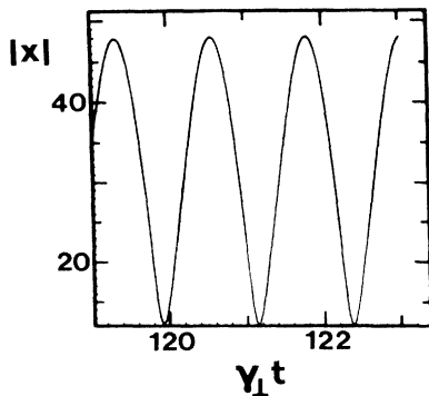
FIG. 6. Self-oscillations predicted by the model (4.2) for C=300 , \Delta=3 , \Theta=-25 , \kappa'=0.4 , \gamma=1.6 , and y=900 . The modulus |x| of the electric field is plotted as a function of \gamma_1 t .
