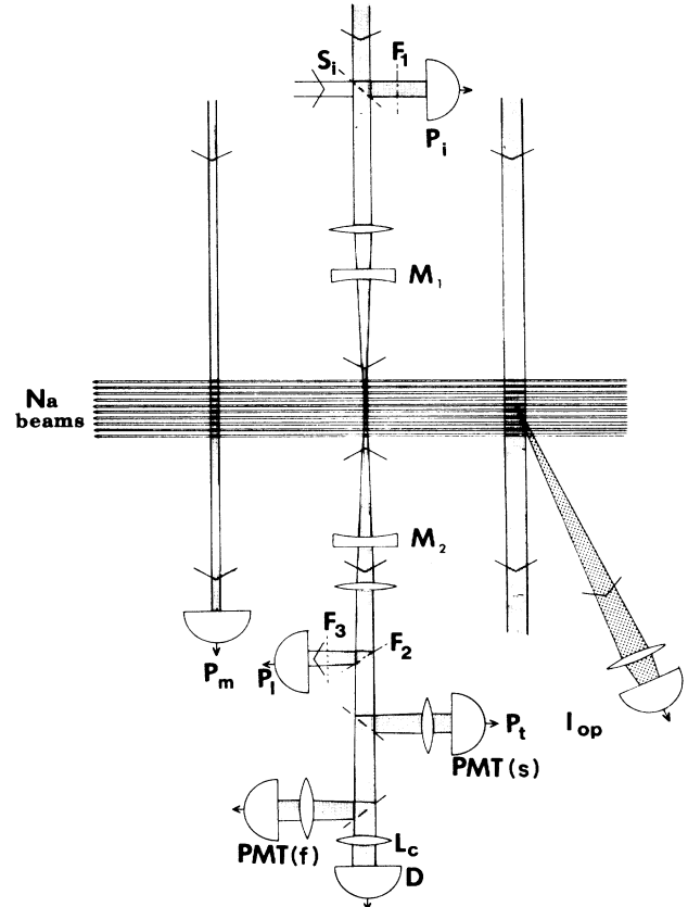
FIG. 10. Experimental setup. Top view: Three laser beams (fine shade) intersect at 90^\circ ten well-collimated atomic beams of sodium. The first beam optically prepumps the atoms but consists of two independent lasers offset by 1.71 GHz to obtain maximum atomic density, with the fluorescence (grainy shade) from one of the center beams ( I_{OP} ) collected onto a photomultiplier tube. The second laser (signal beam) is mode matched to the cavity formed by mirrors M_1 and M_2 . The input power ( P_i ) is measured by splitting a constant fraction onto a photodiode. A second laser, Zeeman-stabilized He-Ne (not shaded), is mixed with the signal beam at the beam splitter S_i ; an interference filter ( F_1 ) is placed in front of the input diode ( P_i ) to pass only 589-nm light. The output power transmitted through the cavity is first incident on a filter ( F_2 ) which passes only 589-nm light and reflects predominantly the 633-nm beam onto a photodiode ( P_1 ) through the filter F_3 for the 633 nm to lock the cavity. Then the 589-nm light is split onto two photomultiplier tubes: PMT(S), which is externally limited in bandwidth (7 MHz) and serves to record the output characteristics of the system P_i , while PMT(f) is a fast photomultiplier whose output is displayed on a spectrum analyzer to identify instabilities. The last part of the output beam is focused with a cylindrical lens L_c onto an array of diodes D to measure the spatial transverse profile of the output field. Further downstream the small-signal absorption is measured with the monitor beam ( P_m ). The transverse dimensions of the laser beams relative to the atomic beams are exaggerated in the figure.
