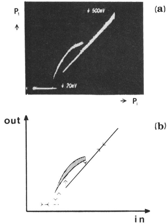
FIG. 21. (a) Input-output characteristics ( P_t vs P_i ) for C=250\pm 50 , \Theta=14\pm 3 , \Delta=-3.0\pm 1.0 , \kappa'=0.4 , and \gamma=1.6 in the ring d cavity, when a hard-mode instability is present, giving rise to a new bistable region associated with the oscillatory state. (b) Explanatory drawing of the instability as an arch separated from the upper branch, the arrows indicating the direction of switching as the input intensity is scanned at a rate of 50 Hz.
