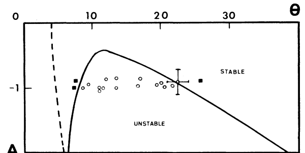
FIG. 17. Domain of instability in the detuning space for C=60\pm 5 , \kappa'=0.5 , and \gamma=1.6 . Open circles indicate instability, closed squares stability. Below the continuous line is the unstable region based on the Gaussian theory, while to the right of the dashed line is the plane-wave prediction of the unstable region. The ring cavity c is used in this measurement. Systematic uncertainties in the detunings are \pm 10\% .
