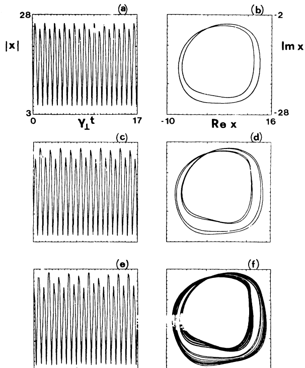
FIG. 2. Self-oscillations from the numerical solution of Eqs. (2.20) for C=400 , \Delta=-1 , \Theta=20 , \kappa'=0.4 , and \gamma=1.76 . (a), (c), and (e) show the normalized transmitted field |x| as a function of \gamma_1 t ; (b), (d), and (f) show the projection of the phase-space trajectory in the plane (\text{Re } x, \text{Im } x) ; (a) period 2 for \gamma = 309.1 ; (b) period 4 for \gamma = 303 ; (c) chaos for \gamma = 297.3 .
