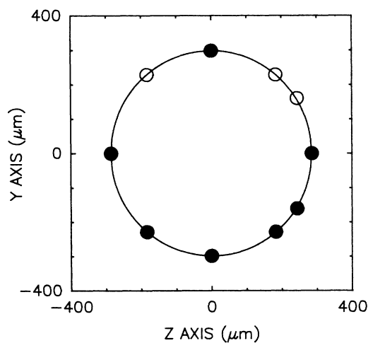
FIG. 11. Boundaries of a {}^9\text{Be}^+ plasma in the y - z plane. The ● data points were measured and the ○ data points were determined by assuming rotational symmetry about the plasma z axis. The ellipse was determined from the end points along the y and z axis. The plasma consisted of 5000 {}^9\text{Be}^+ ions (density of 4.7 \times 10^7 ions/cm ^3 ). The data were taken on trap I at a magnetic field of 1.4 T and axial frequency of \omega_z/2\pi = 290 kHz.
