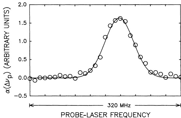
FIG. 13. Graph of \alpha(\Delta\nu_p) as determined from the measured depopulation curve \beta(\Delta\nu_p) along with a Gaussian fit. The full width at half maximum of this resonance is 71.3 MHz. This corresponds to a temperature of 0.11 \pm 0.05 K.
