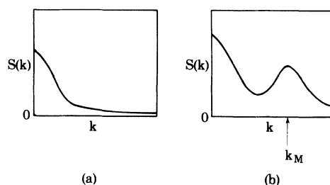
FIG. 3. Schematic plots of the structure factor S(k) vs the magnitude of the wave vector k ( k = |\mathbf{k}| ) in the microemulsion phase. In some cases (a) S(k) displays a maximum at k=0 ; in others (b) S(k) has an additional maximum at k = k_M with k_M^{-1} \approx 100 \text{ \AA} . For more detailed graphs see Ref. 31.
