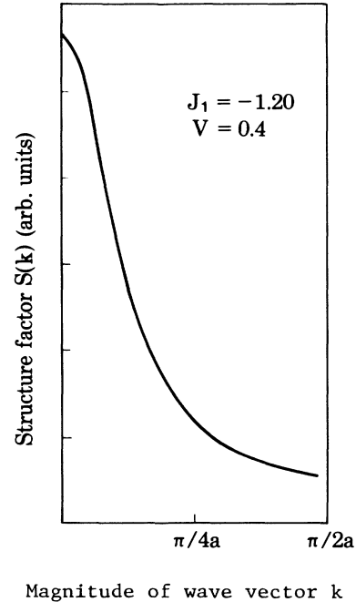
FIG. 6. Oil-water (partial) structure factor of our model for J_1 = -1.20 , V = 0.40 , and T = 0.356 , where a microemulsion phase exists [cf. Fig. 3(a)]. Note that there is no subsidiary maximum. The width of the peak is larger than that for the Ising model at a comparable distance from the transition.
