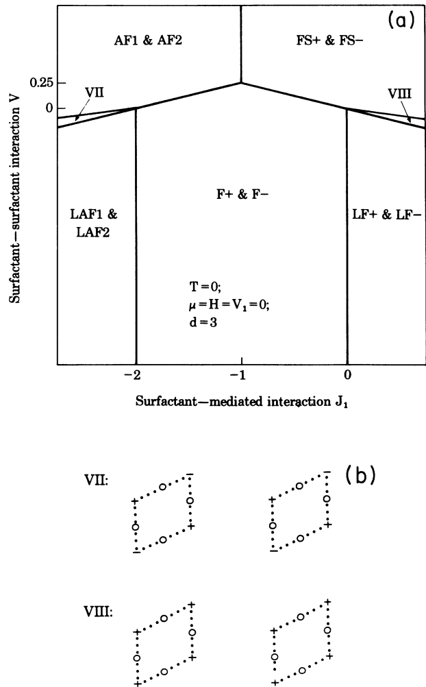
FIG. 10. Zero-temperature phase diagram for model (1) in d = 3 with \mu = H = V_1 = 0 . The phases AF1, AF2, LAF1, LAF2, F+ , F- , FS+, FS-, LF+, and LF- have microstructures which are the natural three-dimensional analogs of the corresponding d = 2 structures displayed in Fig. 9(a). The structures of the phases denoted by VII and VIII are shown in (b).
