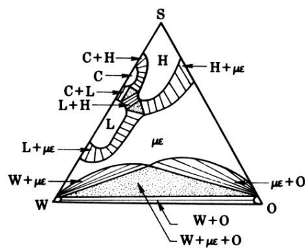
FIG. 2. Schematic phase diagram for an oil-water-surfactant ( O - W - S ) mixture in the composition triangle at fixed temperature. Unshaded areas represent single-phase regimes, areas hatched with tie lines indicate regions of two-phase coexistence, and dotted areas denote three-phase coexistence regions. Oil-rich, water-rich, microemulsion ( \mu\epsilon ), lamellar ( L ), hexagonal ( H ), and cubic ( C ) phases are shown. In laboratory mixtures all these phases might not coexist as shown at one temperature; furthermore, different types of cubic, hexagonal, and lamellar phases might occur. The microstructure of the \mu\epsilon phase varies from the oil-in-water type [Fig. 1(c)] near the water-rich corner, through the bicontinuous type [Fig. 1(e)] in the middle of the triangle, to the water-in-oil type [Fig. 1(d)] near the oil-rich corner.
