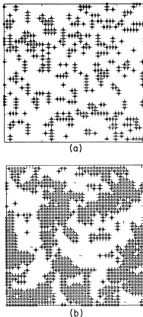
FIG. 13. Representative microstructures in the microemulsion phase from Monte Carlo simulations in d=2 for (a) V_1=0 , \mu=-1.0 , H=-0.05 , V=-0.1 , J_1=-3.0 , and T=0.14 and (b) V_1=\mu=H=0 , V=-0.1 , J_1=-1.8 , and T=0.33 ; in both cases, J=1 and T is approximately 10% above the transition temperature. Note that the clusters in (a) are stringy in contrast to the compact, roughly circular ones in Fig. 4 in another region of parameter space. In (b), the microstructure has large, connected patches of oil and water and is the analog of the d=3 bicontinuous structure. Note that a bicontinuous structure is not possible in two dimensions (Ref. 75).
