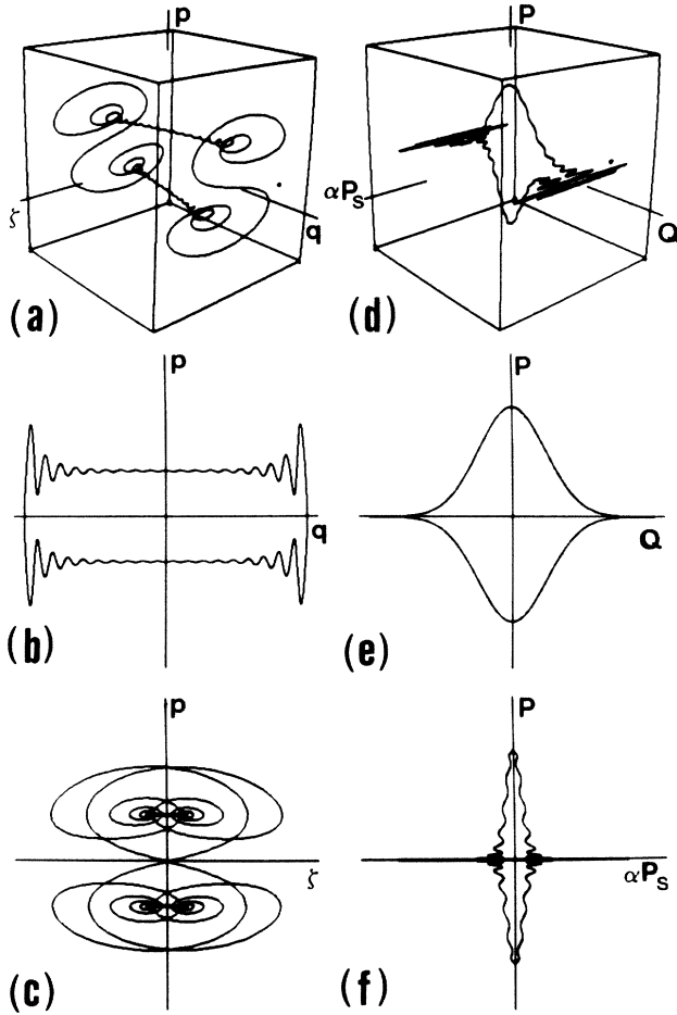
FIG. 7. As in Fig. 2 for \alpha=100 and n=19 . Initial condition: (a)–(c), q_0=0 , p_0=1.0085 , \zeta_0=0 ; (d)–(f), Q_0=0 , P_0=1.0085 , s_0=1 , P_{s0}=0 . Scales: (a)–(c), -4.5 \leq q \leq 4.5 , -3.5 \leq p \leq 3.5 , -20 \leq \zeta \leq 20 ; (d)–(f), -4.5 \leq Q \leq 4.5 , -1.5 \leq P \leq 1.5 , -20 \leq \alpha P_s \leq 20 .
