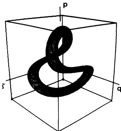
FIG. 1. Regular trajectory of the Nosé oscillator for \alpha = 1 . The q, p, \zeta axes are only drawn outside the cube with the origin at the center. Initial condition: q_0 = 0, p_0 = 2, \zeta_0 = 0 . The range of scales is indicated by the edges of the cube: -1 \leq q \leq 1, -3 \leq p \leq 3, -8 \leq \zeta \leq 8 .
