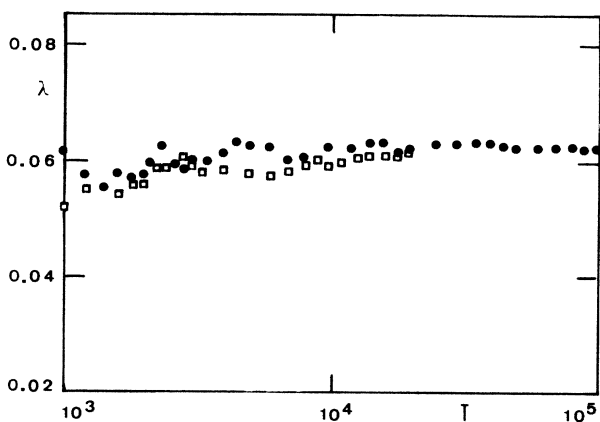
FIG. 14. Convergence of time averages of the Lyapunov exponents of the Nosé oscillator for \alpha=3 ( q_0=0 , p_0=5 , \zeta_0=0 ). Open squares: method employing periodic rescaling of the trajectory offset d of trajectory 2 to d_0=0.003 every 50th time step \Delta t=0.001 . Closed circles: constraint force method Eqs. (25)–(28) for d_0=0.003 and a time step \Delta t=0.01 .
