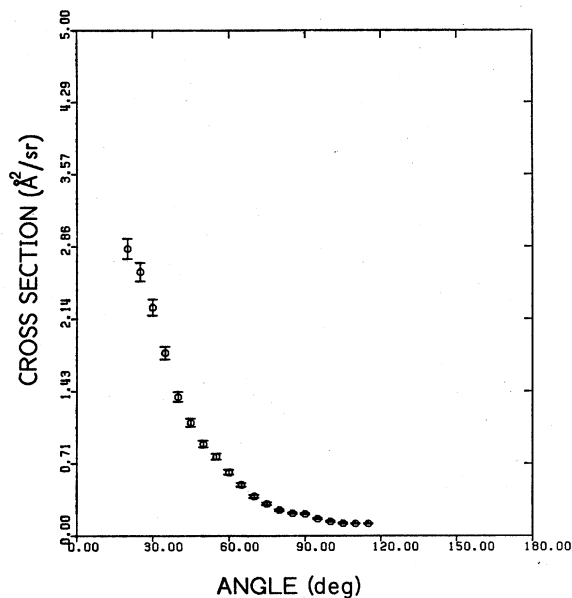
FIG. 9. Differential cross section at 19 eV. \circ , present results.
