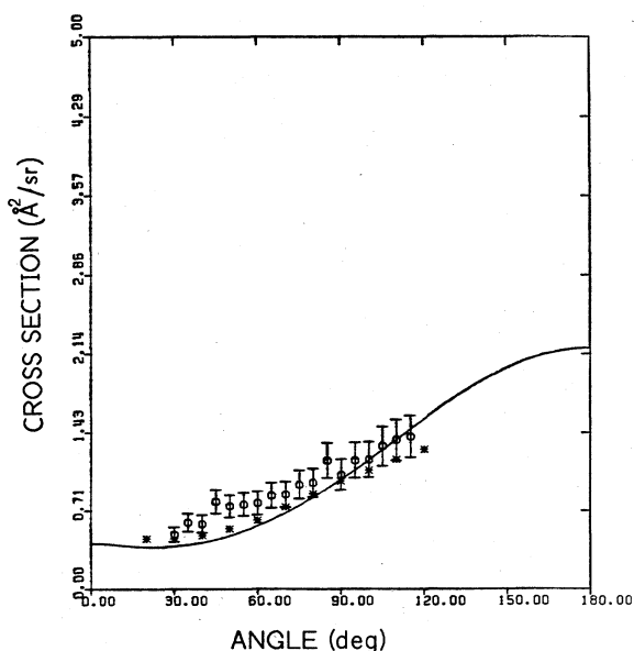
FIG. 1. Differential cross section at 1 eV. \circ , present results; —, Morrison et al. ; *, Linder and Schmidt.
