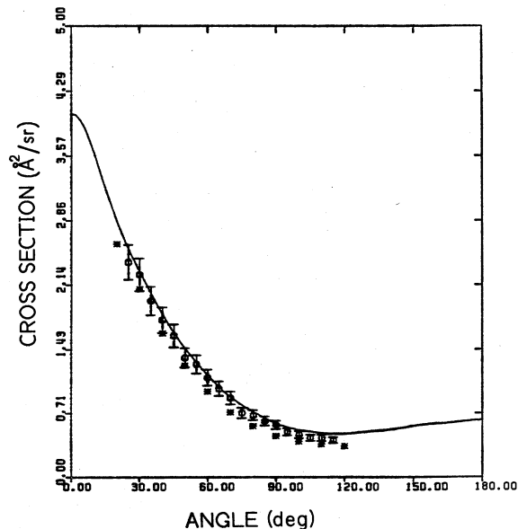
FIG. 6. Differential cross section at 8 eV. \circ , present results; —, Morrison et al. ; *, Linder and Schmidt.
