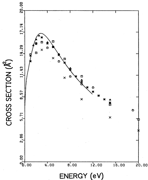
FIG. 10. Integrated total cross section in H_2 . \circ , present results; —, Morrison et al. ; \times , Srivastava et al. and Trajmar et al. ; \square , Shyn and Sharp; \triangle , Dalba et al. ; * , Jones.
