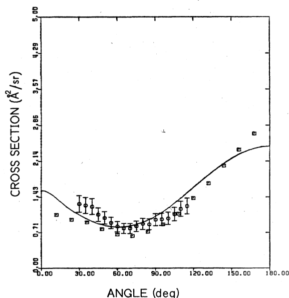
FIG. 2. Differential cross section at 2 eV. \circ , present results; —, Morrison et al. ; \square , Shyn and Sharp.
