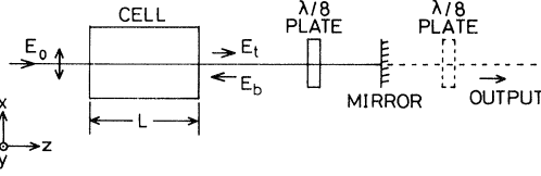
FIG. 1. Optical system exhibiting bistability with symmetry breaking, together with the definition of coordinates. The \lambda/8 plate shown by dashed lines is used to monitor the fields \vec{E}_t and \vec{E}_b .
