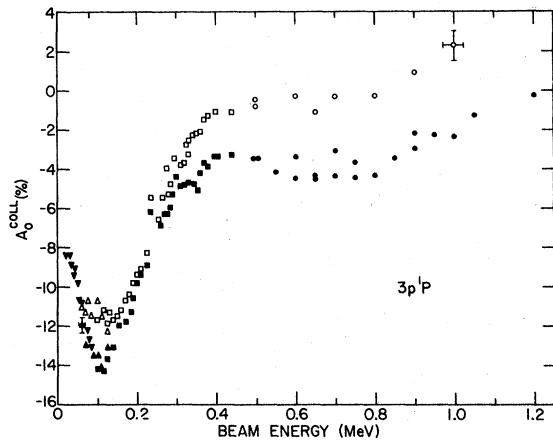
FIG. 1. A_0^{\text{coll}} of the He I 3p^1P state vs beam energy after the foil. Foil areal density: 5\text{--}6.5 \mu\text{g}/\text{cm}^2 . Open points: j = 30 \pm 5 \mu\text{A}/\text{cm}^2 , solid points: j = 6 \pm 2 \mu\text{A}/\text{cm}^2 . Data were taken at Bell Labs (Ref. 17) (upside down triangles), Chicago (triangles), Toledo (squares), Argonne (circles). Alignment error bars are statistical; the error bar at 1.0 MeV includes uncertainty due to the correction for instrumental polarization. Energy error bars represent calibration uncertainty.
