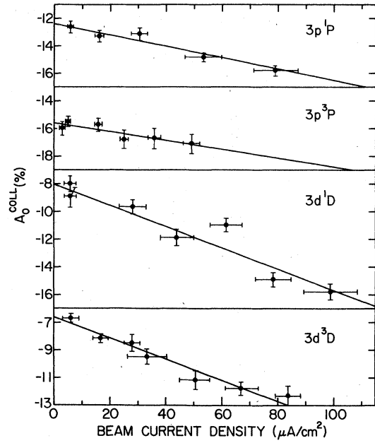
FIG. 5. A_0^{\text{coll}}(0) vs beam-current density for the n = 3 He I states at 125-keV postfoil energy. Beam-current error bars correspond to beam fluctuations during the run. Slope of indicated line = S_j .
