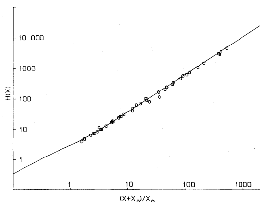
FIG. 3. Graph of the experimental values of h(x) for xenon [dots], as calculated from Levelt Sengers et al. (Ref. 10), vs the theoretical value of h(x) calculated from Eq. (11) [line].
