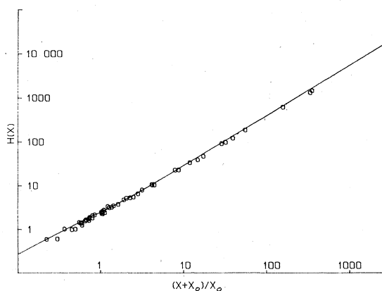
FIG. 1. Graph of the experimental values of h(x) for helium-4 [dots], as calculated from Levelt Sengers et al. (Ref. 10), vs the theoretical value of h(x) calculated from Eq. (11) [line].
