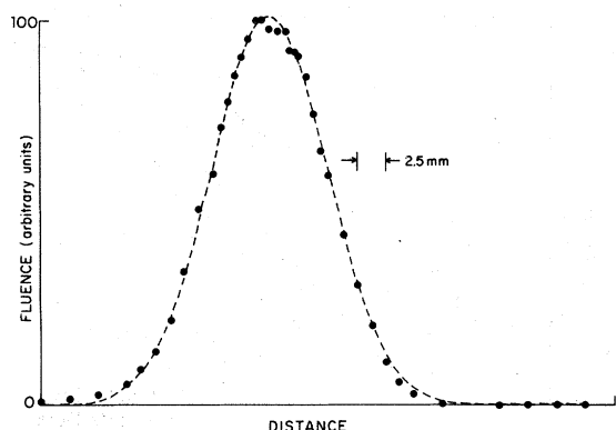
FIG. 5. Measured intensity profile of the incident laser pulses. The points represent the light intensity observed through a 50- \mu m pinhole translated across the beam. The curve is the best-fit Gaussian describing the position of the points on the graph. By this method we accurately determined that our laser beams were Gaussian, and measured the exact size of the beam.
