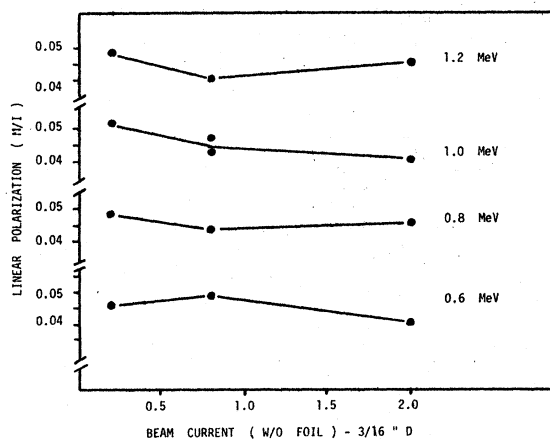
FIG. 4. Linear polarization fraction ( M/I ) of the 3568-Å Ne II 3s\ ^2D_{5/2} = 3p\ ^2F_{7/2} transition excited by a 5 \pm 2\text{-}\mu\text{g cm}^{-2} carbon foil at ion energies of 0.6–1.2 MeV and beam currents of 0.5–2.0 A ( j = 3-10\ \mu\text{A cm}^{-2} ).
