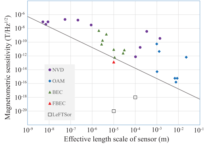
FIG. 1. Summary of the size and sensitivity of spin-based magnetometers. Experimentally demonstrated magnetometers are represented by closed markers and projected sensitivity of proposed magnetometers are represented by open markers. The gray line indicates the energy resolution limit described by Eq. (4). The purple circles correspond to nitrogen-vacancy diamond (NVD) magnetometers [164–171], the green triangles correspond to atomic Bose-Einstein condensate magnetometers [150,172–179], and the blue diamonds correspond to optical atomic magnetometers (OAM) [149,180–186]. The red triangle represents the sensitivity of the recently demonstrated single-domain ferromagnetic BEC magnetometer (FBEC) that surpasses the ERL [187]. Levitated ferromagnetic torque sensors, represented by the open black squares, are predicted to surpass the ERL by many orders of magnitude [18,19]. This figure has been adapted with permission from Ref. [162]; it does not include non-spin-based magnetic sensors based on, for example, superconducting quantum interference devices.
