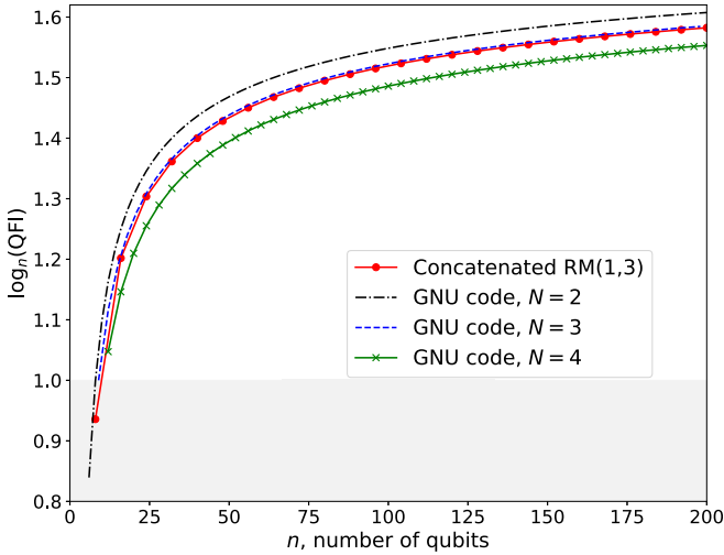
FIG. 2. We plot lower bounds on \log_n(\text{QFI}) for various code-inspired probe states for the robust quantum metrology problem. We compare the lower bounds that we have for the concatenated RM(1,3) code with that of previously studied GNU probe states [22] after one erasure error has occurred. Whenever the lower bound is above one, there is a quantum advantage in using these code-inspired probe states.
