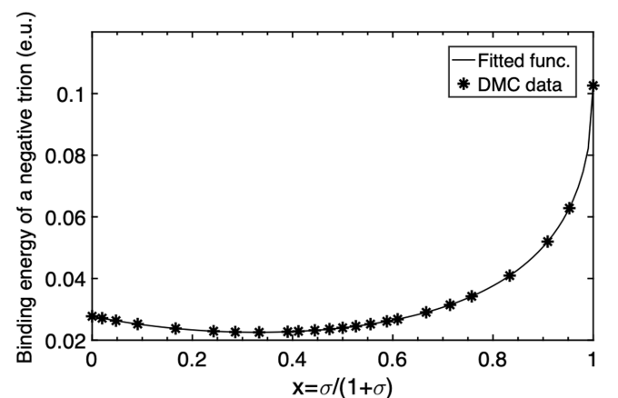
FIG. 2. DMC binding energies of negative trions against rescaled mass ratio x = \sigma/(1 + \sigma) . The solid line shows the fit of Eq. (17).
