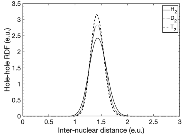
FIG. 9. Nucleus-nucleus RDF 4\pi r^2 g_{hh}(r) for three dihydrogen molecules ( H_2 , D_2 , and T_2 ) vs the nucleus-nucleus distance.
