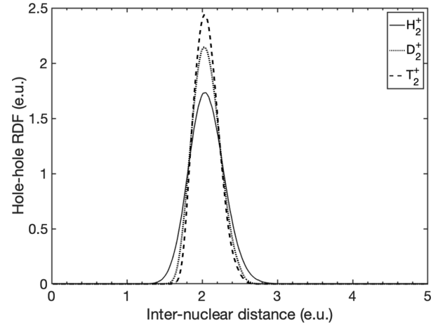
FIG. 4. Nucleus-nucleus RDF 4\pi r^2 g_{\text{hh}}(r) for three dihydrogen cations ( \text{H}_2^+ , \text{D}_2^+ , and \text{T}_2^+ ) vs the nucleus-nucleus distance.
