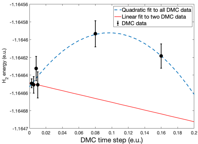
FIG. 13. As Fig. 12, but for an H_2 molecule. The DMC energies extrapolated to zero time step using quadratic and linear fits are -1.164653(5) and -1.164649(8) e.u., respectively.
