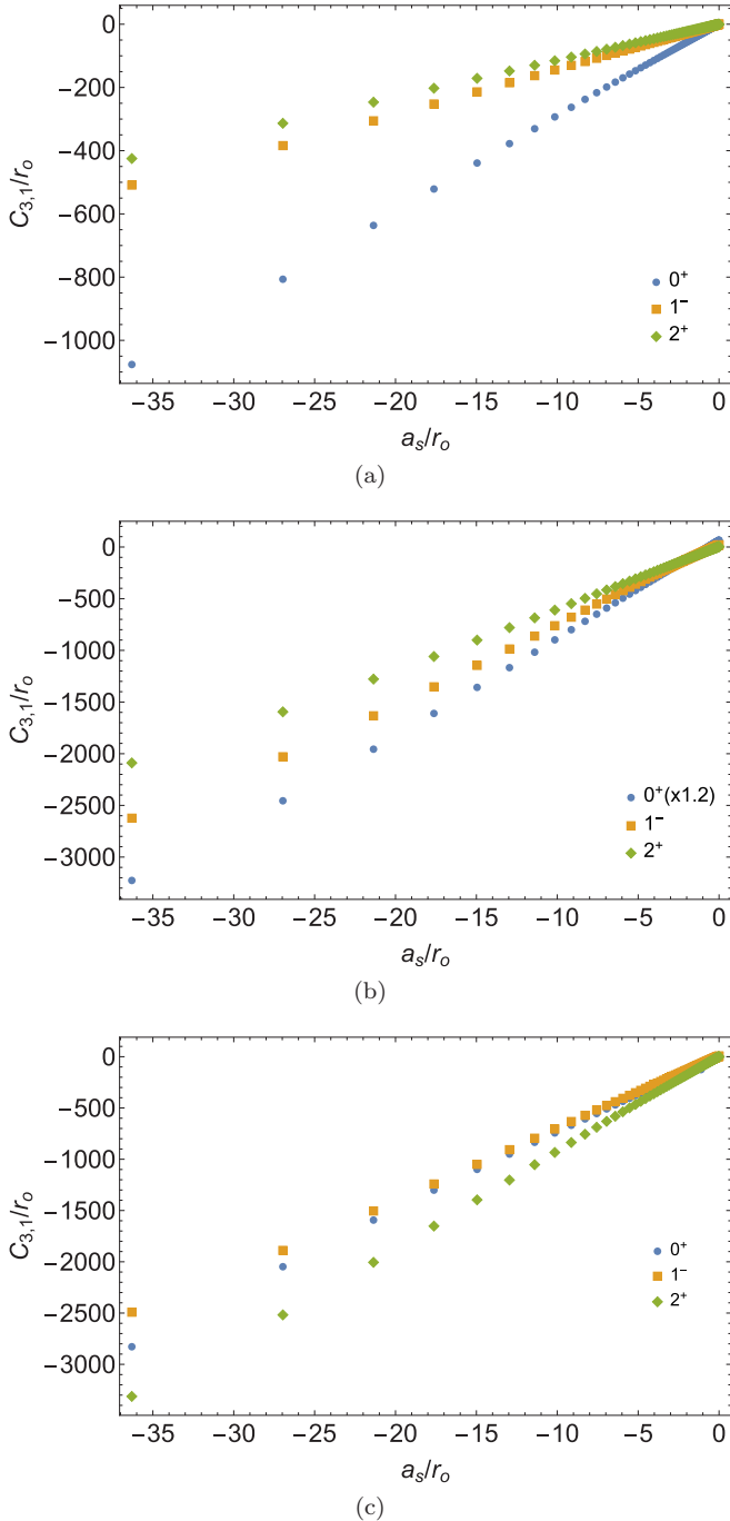
FIG. 6. The long-range coefficient C_{3,1}/r_0 versus a_s/r_0 in the lowest Born-Oppenheimer potential for the (a) ( \uparrow\uparrow\downarrow ), (b) ( \uparrow\downarrow\downarrow ), and (c) ( \uparrow\uparrow\downarrow ) equal-mass systems for the symmetries L^\pi=0^+ (circles), 1^- (squares), and 2^+ (diamonds). For values of the s -wave scattering length near the unitary limit ( |a_s/r_0| > 10 ), C_{3,v} grows in proportion to a_s , in accordance with Eq. (7). These results are for a single Gaussian two-body interaction of width r_0 . The data for the other hyperspherical channels yield qualitatively similar results to the lowest channel in each symmetry, and thus are not shown here.
