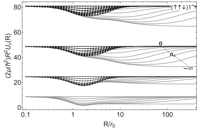
FIG. 4. The lowest few Born-Oppenheimer potential curves for the ( \uparrow\uparrow\downarrow ) equal-mass three-body system are shown for the 1^- symmetry. The solid curves correspond to potentials that exhibit a reduced value of l_{\text{eff}} at the unitary limit for large hyperradius, whereas the dashed potentials go to the noninteracting potentials at large hyperradius. The strength of the two-body interactions between all particles is rescaled from the noninteracting limit up to the s -wave unitary limit ( a_s \rightarrow -\infty ). For each set of curves representing a different channel v , an increase in scattering length on the negative side corresponds to a curve in the set. From highest to lowest, the highest curve is the noninteracting potential, the lowest is the hyperradial potential at the s -wave unitary limit, and a potential in between is for a finite scattering length. The hyperradius has been rescaled by the range of the Gaussian interaction r_0 . The structure of the potential curves for different systems and symmetries is qualitatively similar to the potentials shown here, and thus are not shown.
