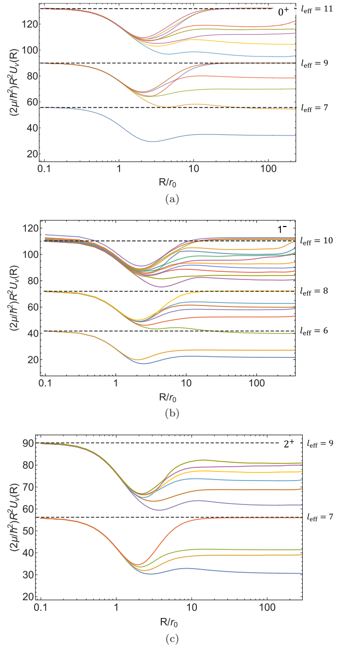
FIG. 3. The lowest few Born-Oppenheimer potential curves for the (\uparrow\uparrow\uparrow\downarrow) equal-mass four-body system are shown for the symmetries (a) L^\pi = 0^+ , (b) L^\pi = 1^- , and (c) L^\pi = 2^+ . Each curve represents a different hyperradial potential with channel index \nu that increases from the lowest to highest curve. The strength of the two-body interaction between all particles is scaled give an infinite s -wave scattering length. The horizontal dashed lines represent the noninteracting rescaled potentials with their effective angular momentum quantum numbers l_{\text{eff}} labeled to the right. The hyperradius has been rescaled by the range of the Gaussian interaction r_0 . For some of the higher degenerate channels, the potentials deviate at small hyperradius due to incomplete basis set convergence.
