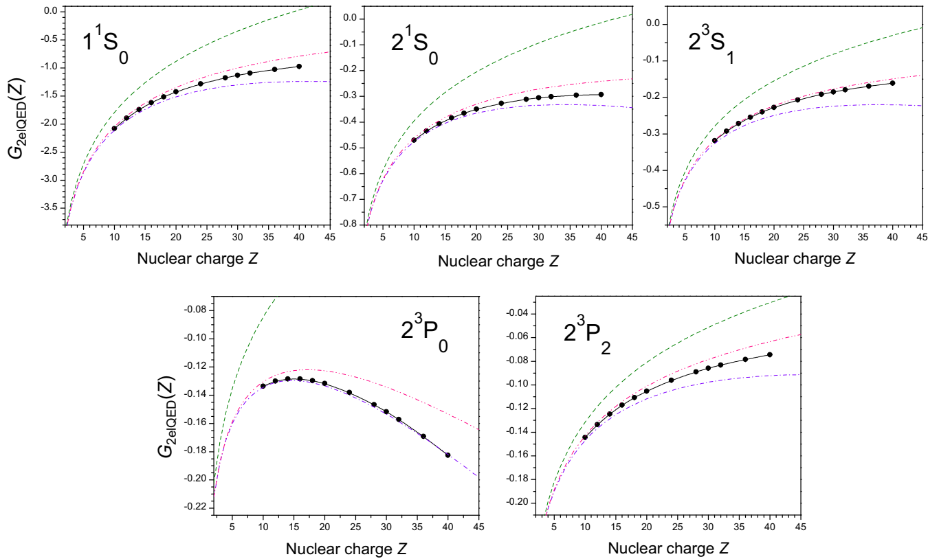
FIG. 1. The two-electron QED correction for nonmixing states of He-like ions, as a function of the nuclear charge number Z , in terms of the function G_{2\text{elQED}} defined by Eq. (21). The dots and solid line (black) present results of all-order numerical calculation. The dashed line (green) shows the contribution of the leading Z\alpha -expansion term of order \alpha^2(Z\alpha)^3 ; the dashed-dotted line (violet) is the contribution of two first Z\alpha -expansion terms of order \alpha^2(Z\alpha)^3 and \alpha^2(Z\alpha)^4 ; and the double-dotted dashed line (pink) shows the contribution of two first Z\alpha -expansion terms plus the hydrogenic estimate of the higher-order terms.
