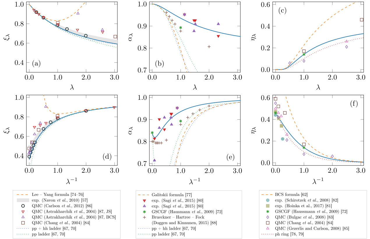
FIG. 1. Dimensionless ground-state energy [first column (a), (d)], effective mass [second column (b), (e)], and pairing gap function [third column (c), (f)] for spin-symmetric infinite dilute systems of identical fermions with negative s -wave scattering length at zero-temperature as a function of \lambda [first row (a), (b), (c)] and \lambda^{-1} [second row (d), (e), (f)]. The blue solid line correspond to our parametrization of the functional defined by Eq. (4): the ground-state energy and the effective mass correspond to the APS functional [70] by setting x \simeq -0.75 adjusted to reproduce the result of Ref. [72, green asterisks] at unitarity, and the pairing gap function is given by Eq. (17). For reference, we display the second-order MBPT results, known as the Lee-Yang [74–76] and Galitskii formula [77] for the ground-state energy and the effective mass, respectively, and the BCS equation [62] (orange dashed lines) as well as the ladder resummation of the particle-particle [67,70] (green dotted lines), particle-particle and hole-hole [67,70] (blue dotted lines), and particle-hole channels [78,79] (red dotted line). We show also various experimental results from Ref. [80, triangles], Ref. [81, light green squares], Ref. [82, light blue circles], Ref. [57, gray area], QMC calculations of Ref. [83, purple open diamonds], Ref. [84, brown open squares], Ref. [85, pink open up-triangles], Ref. [86, black open circles], Ref. [87, red open down-triangles (Jastrow-Slater trial wave function) and purple open up-triangles (BCS trial wave function)], and Brueckner-Hartree-Fock calculation [88, plus crosses].
