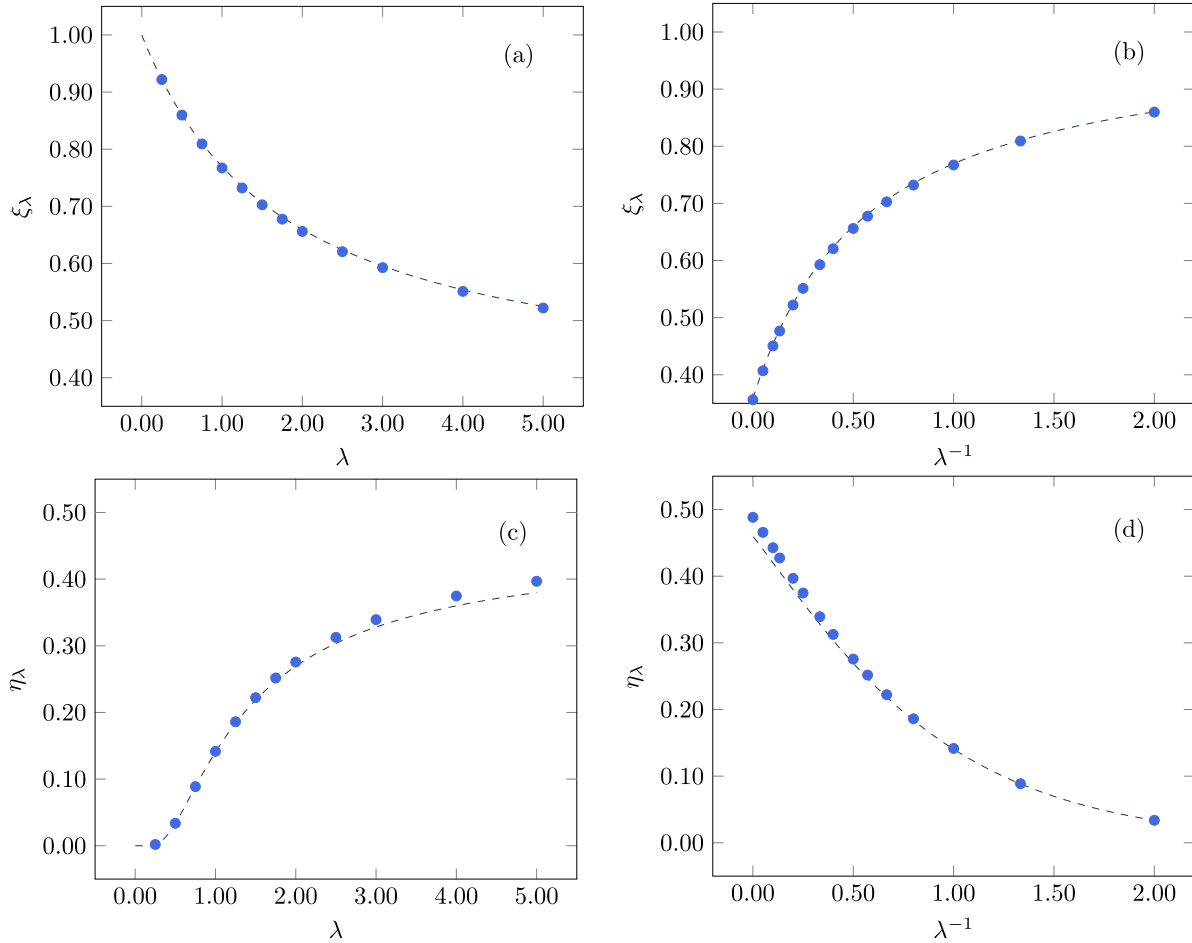
FIG. 4. Dimensionless ground-state energy [respectively, pairing gap function] as a function of \lambda (a) [respectively, (c)] and of \lambda^{-1} (b) [respectively, (d)] obtained by solving numerically the BdG equations associated to the constructed functional together with the regularization scheme defined by Eq. (20) [blue filled circle]. The computation was executed on a spatial mesh of size 80^3 with lattice spacing dx = 1 , and density was set to satisfy k_F = 1 . The dashed black line corresponds to the analytical parametrization of the APS[ x, y, z ] functional that was used as the input for the induction procedure.
