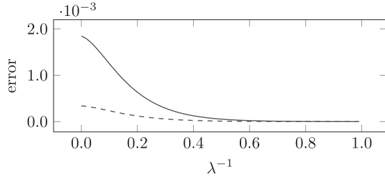
FIG. 2. Numerical error using perturbative solutions given by Eq. (13) in Eq. (12) as a function of \lambda^{-1} . The solid and the dashed lines show the absolute difference of the right-hand side and left-hand side of Eqs. (12a) and (12b), respectively. Note that the perturbative expansion becomes less accurate, but still very reasonable, close to the unitary regime because \eta_\infty/\alpha_\infty \sim 0.6 .
