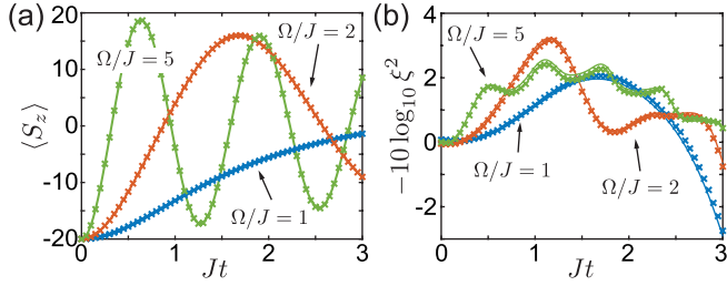
FIG. 3. Plot of the time evolution of (a) the magnetization \langle S_z \rangle and (b) the squeezing parameter \xi^2 of a driven spin ensemble with different driving strengths \Omega/J = 1, 2, 5 and individual dephasing with rate \Gamma_\phi/J = 0.2 . Initially, all the spins are polarized along the negative z axis, |\Psi_0\rangle = \prod_i |\downarrow\rangle_i . In both plots, N = 40 and all-to-all interactions ( \alpha = 0 ) are assumed. The solid lines are obtained from an exact integration of the master equation exploiting permutational invariance, while the crosses are obtained from a DDTWA simulation with n_t = 10000 trajectories.
