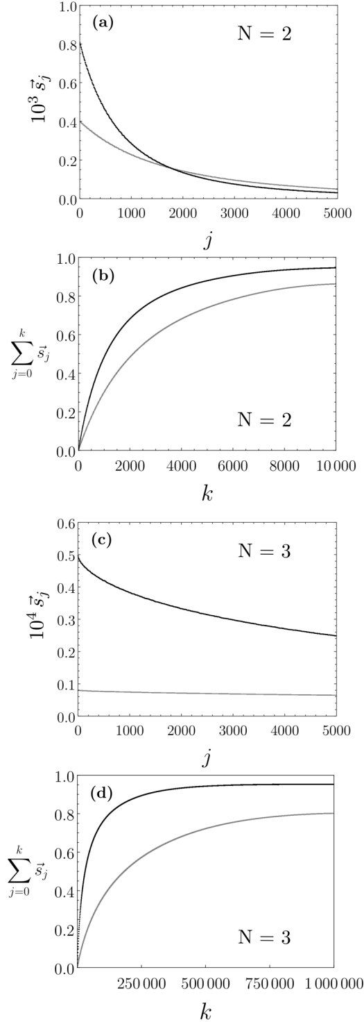
FIG. 3. (a) Schmidt coefficients distribution \bar{s}^i (gray squares) and \bar{s}^f (black dots) for \lambda L = 200 and N = 2 . (b) Sum of the first k ordered Schmidt coefficients for each of the distributions in (a) showing the numerical verification of the majorization criterion ( \bar{s}^i \prec \bar{s}^f ) up to 10^4 coefficients for N = 2 with the same color scheme as before. (c) Same as (a) for N = 3 . (d) Same as (b) for N = 3 and 10^6 coefficients.
