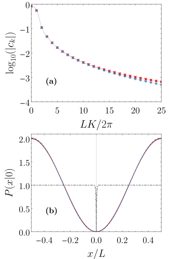
FIG. 1. (a) Logarithm of the absolute values of the coefficients obtained from the numerical calculation for \lambda L = 200 (blue seven-pointed stars) and from the analytic expression for infinite attractive interaction (red four-pointed stars). (b) Probability of finding a particle of kind a at position x given that another particle of the same kind was found at position 0 obtained from the numerical calculation for \lambda L = 200 (dashed blue line) and from the analytical solution (solid red line) in Eq. (31). The probability given by the coboson ansatz [see Eq. (24)] is shown by the dot-dashed gray line.
