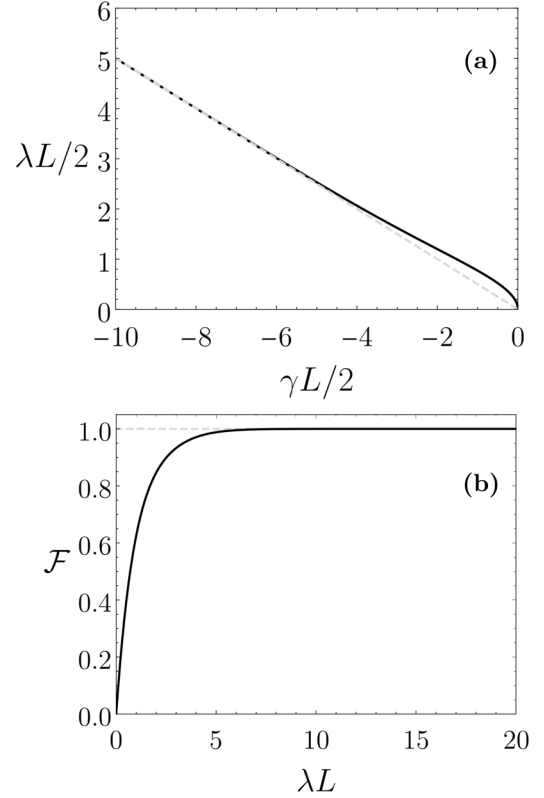
FIG. 2. (a) Energy parameter \lambda vs the interaction strength \gamma (black solid curve) and the corresponding approximation [see Eq. (A7)] for \gamma \gg 1 (gray dashed line). (b) Fidelity between the state and its approximation for \gamma \gg 1 as a function of the interaction strength.
