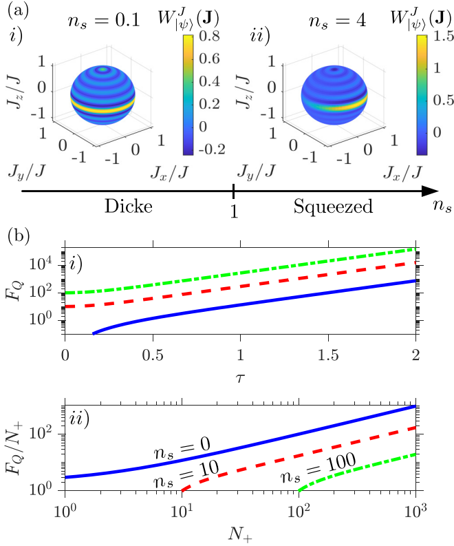
FIG. 2. (a) SU(2) Wigner distributions W_{|\psi\rangle}^J(\mathbf{J}) for |\psi_t^s\rangle projected into the J = 10 sector for (i) n_s = 0.1 and (ii) n_s = 4 and fixed N_+ = 10^2 . The distributions are renormalized to account for the projection onto the J = 10 sector. (b) QFI, F_Q , as a function of (i) collision duration \tau and (ii) total population N_+ in m_F = \pm 1 modes. In panel (ii), we plot the normalized QFI per particle, where F_Q/N_+ > 1 indicates sub-SQL sensitivity when only the m_F = \pm 1 populations are considered. Predictions are from the undepleted pump approximation, Eq. (17), with initial seed occupation: n_s = 0 (blue solid lines), n_s = 10 (red dashed lines), and n_s = 100 (green dot-dashed lines).
