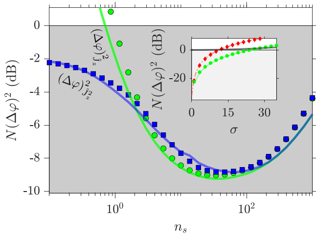
FIG. 6. Best achievable sensitivity as a function of seed n_s after optimization over interaction time \tau . The sensitivity is rescaled relative to the absolute SQL (\Delta\varphi)_{\text{SQL}}^2 = 1/N . We compare results of full numerical simulations for a measurement of \hat{J}_z (green circles) or \hat{J}_z^2 (blue squares) with analytic expressions (corresponding blue and green lines overlaying the markers) derived from the undepleted pump approximation [e.g., optimization of Eq. (20)] with \bar{n} matched to numerical simulations. We include fixed detection noise \sigma = 8 . Inset: Sensitivity as a function of \sigma obtained from numerical calculations with optimally chosen initial seed n_s (green squares) compared to n_s = 0 prediction (red data). Lines (red dashed for n_s = 0 and green solid for n_s \neq 0 ) are analytic predictions from undepleted pump approximation with matching N_+ .
