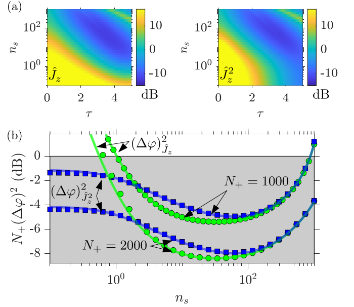
FIG. 5. (a) Normalized sensitivity N_+(\Delta\phi)^2 obtained from full quantum dynamics [governed by \hat{H} , Eq. (1)] of an initial BEC of N = 10^4 atoms as a function of initial seed occupation n_s and interaction time \tau . Measurement signals are indicated on panels. Note that the plotted data saturates the color scale in lower left corner of panels (i.e., N_+(\Delta\phi)^2 > 10 dB). (b) Optimal sensitivity as a function of seed n_s , with \tau chosen such that N_+ = 1000 or 2000 (indicated by arrows). Markers indicate results of full numerical simulations for a measurement of \hat{J}_z (circles) or \hat{J}_z^2 (squares), while the tracking solid lines are equivalent analytic predictions from the undepleted pump approximation [e.g., Eq. (20)] with \bar{n} and n_s chosen to match numerical results. In all panels of (a) and (b), we include fixed detection noise \sigma = 8 .
