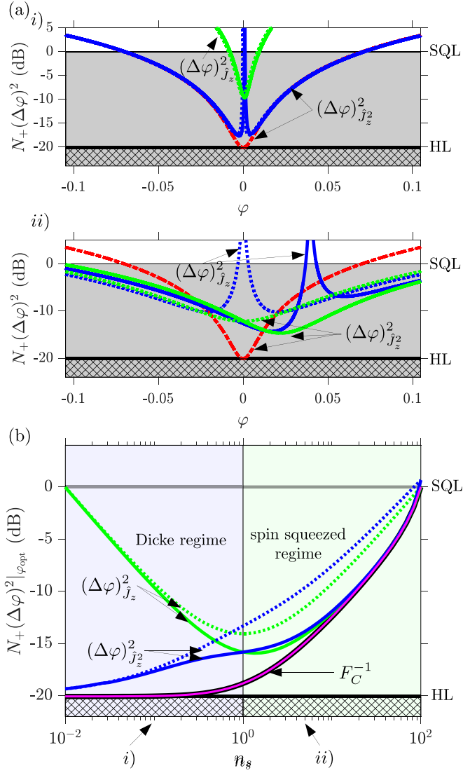
FIG. 3. (a) Example interferometric sensitivities as a function of phase shift \varphi for different initial conditions: (i) n_s = 0.1 and (ii) n_s = 4 . The sensitivities are computed from measurements of \hat{J}_z (green lines) and \hat{J}_z^2 (blue lines) as labeled. Line style indicates single (solid) and dual seed (dotted) initial conditions. We also plot the case of n_s = 0 with a \hat{J}_z^2 measurement (red dot-dashed line), which saturates the HL, as a reference in both panels. For all data, \theta_s is optimally chosen (see main text) and N_+ = 10^2 is fixed. (b) Optimal sensitivity as a function of initial seed occupation n_s and N_+ = 10^2 . We indicate with arrows the results of measurements of \hat{J}_z (green lines) and \hat{J}_z^2 (blue lines) against the CFI F_C^{-1} [Eq. (27), narrow magenta line] that also saturates the QCRB [Eq. (17), thick black line underlying CFI]. The line styles indicate single (solid) and dual seed (dotted) initial conditions. For clarity, we also indicate the Heisenberg (HL) and standard quantum limits (SQL) for N_+ = 10^2 in all panels.
