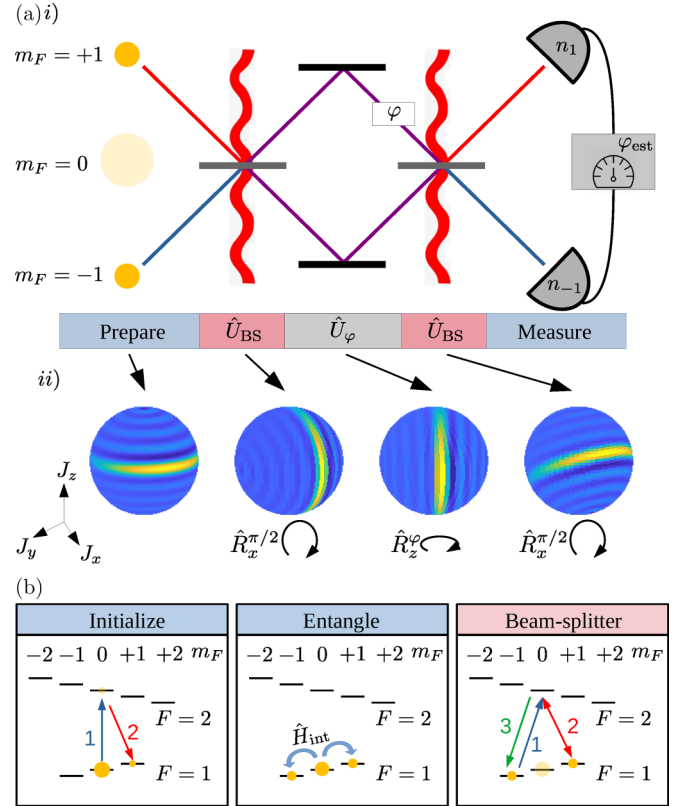
FIG. 1. (a) Interferometric sequence. (i) Illustration of a Mach-Zehnder scheme, where entangled pairs of m_F = \pm 1 atoms are the input state of the upper and lower paths. Beam splitters are realized by coherently mixing the m_F = \pm 1 modes [see (b)] and a relative phase shift \varphi is imprinted. Accruing a phase shift due to gravity requires combining state-dependent momentum kicks imparted by laser pulses (red curves) with the internal-state beam splitters. An estimate of \varphi is obtained by measuring populations \hat{n}_{\pm 1} at the outputs. (ii) In an equivalent Ramsey sequence, the beam-splitter and phase-shift operations correspond to rotations (axes indicated) of the quantum state on a collective Bloch sphere, illustrated using the Wigner phase-space distribution of an example squeezed state (see Sec. III for details). (b) Example internal state dynamics for F = 1 sodium spinor BEC. Initialize: Coherent seeding is implemented via microwave pulses resonantly tuned to an ancillary F = 2 manifold that transfer a fraction of the total population to the m_F = \pm 1 modes. Pulse 1 transfers n_s atoms from (F, m_F) = (1, 0) \rightarrow (2, 0) and pulse 2 completes the transfer to (1, 1) [split equally to (1, -1) for dual seeding]. Entangle: Subsequent spin-changing collisions between m_F = 0 atoms produce entangled pairs in m_F = \pm 1 to realize |\psi_i^{s,d}\rangle . Beam splitter: Coherent mixing of the m_F = \pm 1 modes is also implemented via resonant microwaves. Pulse 1 transfers the entire population from (1, -1) \rightarrow (2, 0) before pulse 2 implements coherent 50:50 mixing of (2, 0) \leftrightarrow (1, 1) . Finally, pulse 3 returns the remaining population from (2, 0) \rightarrow (1, -1) .
