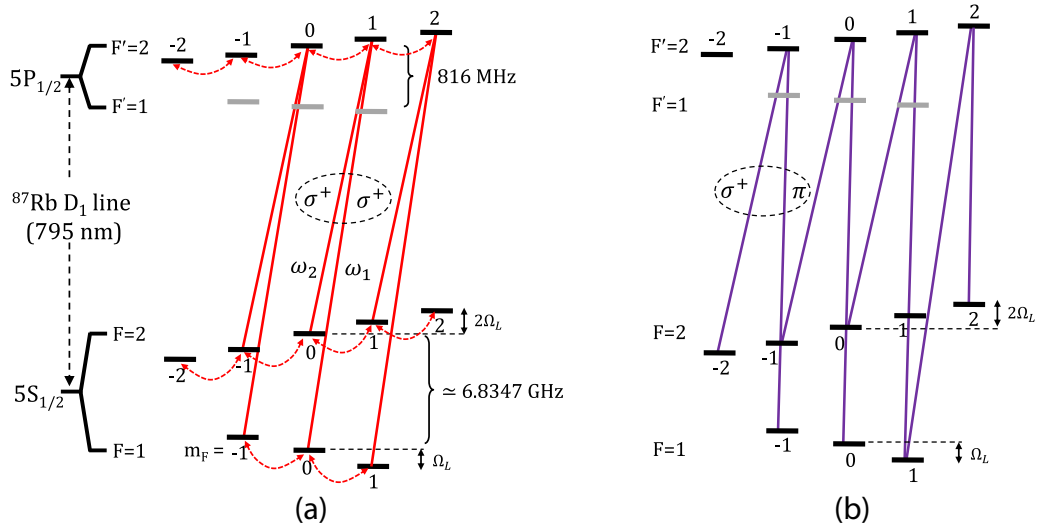
FIG. 2. Energy diagrams showing \Lambda systems formed due to interaction of the modulated bichromatic \sigma^+ polarized laser field with ^{87}\text{Rb} D_1 manifold in the presence of a magnetic field \vec{B} . Resonant two-photon excitation with |F' = 2\rangle excited state is considered here. The formation of \Lambda systems in (a) are shown by considering the z axis as the quantization axis, and in (b), by considering the direction of \vec{B} as the quantization axis. In (b), \Lambda systems formed by the (\sigma^+, \pi) combination are shown. The resonant frequency for each \Lambda system can be inferred from the diagrams.
