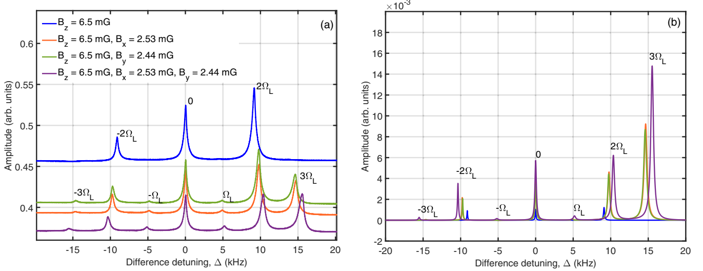
FIG. 3. (a) Experimental CPT spectra acquired using continuous resonant two-photon excitation with |F' = 2\rangle excited state and \sigma^+ polarized light fields. (b) Theoretical CPT spectra calculated using similar excitation conditions as in the experiment. A total optical power of 100 \mu\text{W} is used in the laser beam. Different colors in CPT spectra are chosen for different external magnetic fields. The following parameters are used in our simulations: \Omega_1 = \Omega_2 = \Gamma/180 and spontaneous decay rate \Gamma = 6 MHz for ^{87}\text{Rb} atoms.
