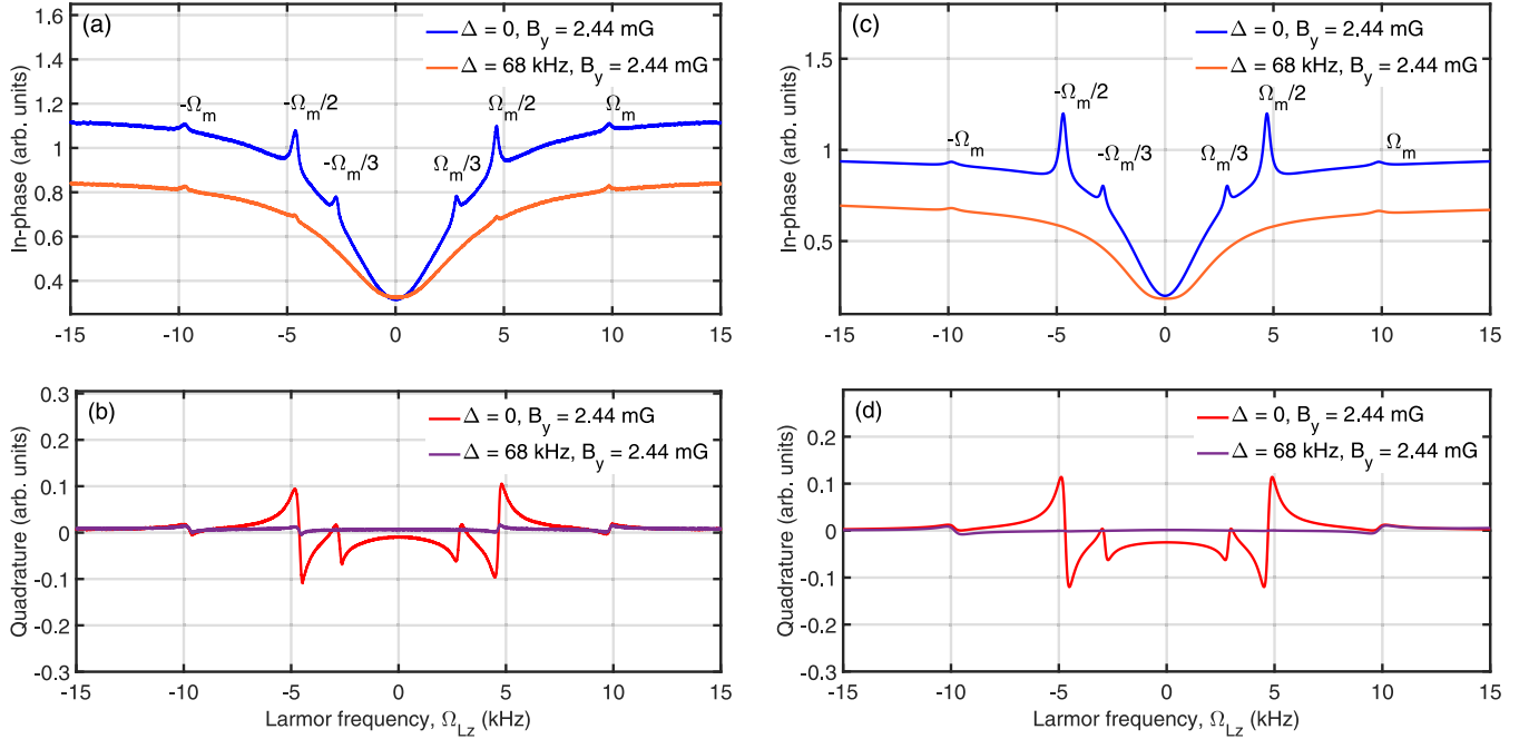
FIG. 5. (a), (b) Experimental magnetic resonance spectra acquired by scanning the longitudinal field B_z and simultaneously applying a constant transverse field B_y (=2.44 mG). (c), (d) Corresponding spectra calculated using our theoretical model. A modulated bichromatic laser beam ( \Omega_m = 10 kHz and 50% duty cycle) with \sigma^+ polarization and in resonance with |F' = 2\rangle excited state is used.
