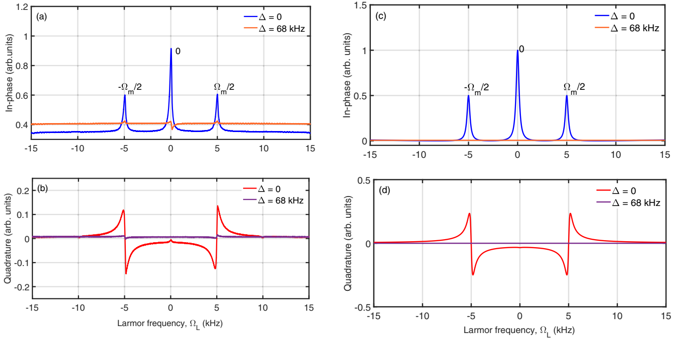
FIG. 4. (a), (b) Experimental magnetic resonance spectra ( I and Q components) acquired by scanning the longitudinal field B_z (or \Omega_L ) around zero value. A modulated bichromatic laser beam ( \Omega_m = 10 kHz and 50% duty cycle) with \sigma^+ polarization and in resonance with |F' = 2\rangle excited state is used. (c), (d) Magnetic resonance spectra calculated using our theoretical model. Difference detuning \Delta = 0 corresponds to synchronous CPT and \Delta = 68 kHz is considered analogous to SOP. Parameters used in our simulations are the same as those in Fig. 3.
