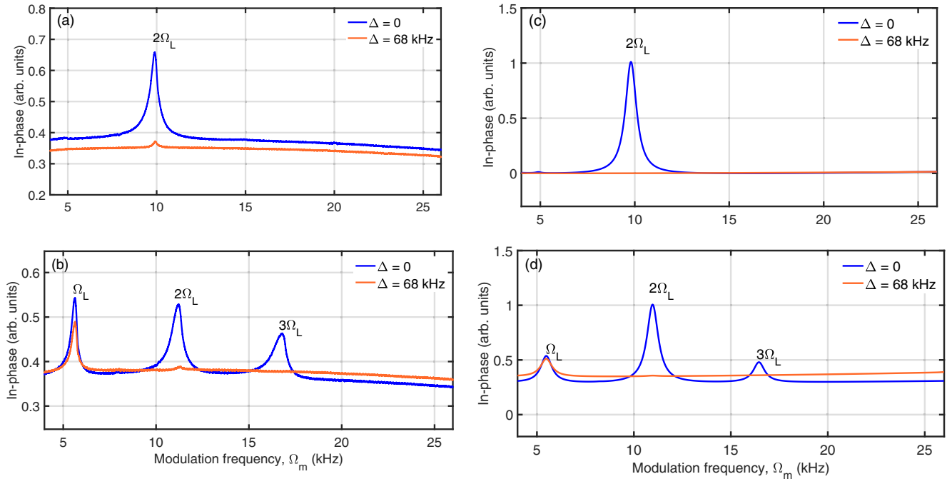
FIG. 8. (a), (b) Experimentally acquired in-phase components of magnetic resonance signals for constant magnetic fields: (a) B_z = 7 mG and (b) B_x = 2.54 mG, B_y = 2.44 mG, and B_z = 7 mG. (c), (d) Corresponding theoretical results. A modulated bichromatic laser beam with \sigma^+ polarization and in resonance with the |F' = 2\rangle excited state is used in this case.
