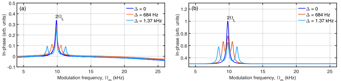
FIG. 7. (a) Experimentally acquired in-phase component of the magnetic resonance signal, obtained by using a constant magnetic field B_z = 7 mG and scanning the laser modulation frequency \Omega_m . (b) Corresponding theoretical results. A modulated bichromatic laser beam with linear polarization and in resonance with the |F' = 1\rangle excited state is used.
