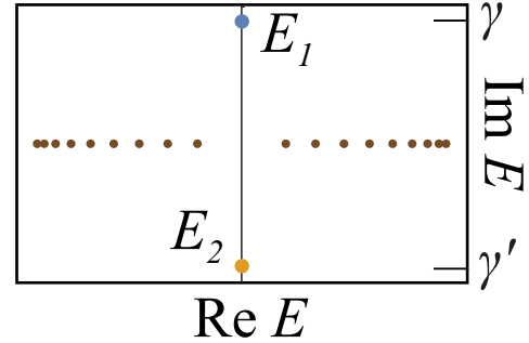
FIG. 3. Complex energy spectrum of a finite system with closed boundary conditions, based on model (1) with parameters as defined in Eqs. (15) and (16). The two states with purely imaginary energies E_1 and E_2 arise from the topological edge states of the system, which exist for dimerization parameter \kappa < 1 , and are well isolated from other states on the imaginary axis as long as the gain-loss contrast |\gamma - \gamma'| < |2w(1 - \kappa)| . In the figure, \kappa = 0.4 and \gamma - \gamma' = w(\kappa - 1) . Notably, this spectrum is independent of the nonreciprocity parameter d , which, however, determines the edge where these states are localized (see phase diagram in Fig. 4).
