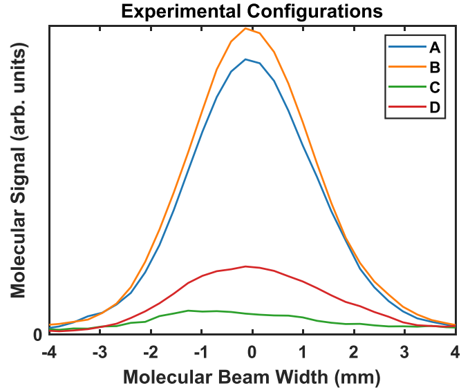
FIG. 6. Molecular signal under the four experimental configurations to determine the repump fraction of \tilde{X}(01^1_0) . This depicts how substantial fractions of molecular population may be optically pumped via small decay pathways during repeated photon cycling.
