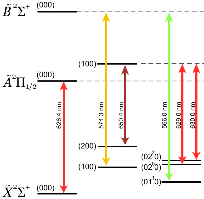
FIG. 1. Vibrational structure of CaOH and laser cooling scheme experimentally considered in this work.
