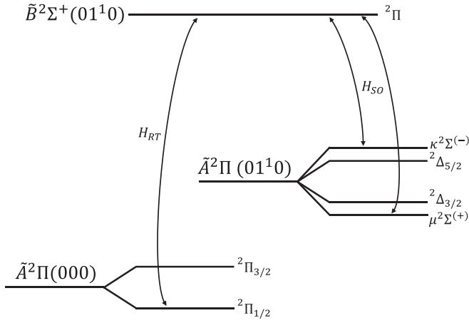
FIG. 7. Illustration of the processes leading to vibronic mixing of \tilde{A}^2\Pi(000) with states of \ell = 1 character. First-order mixing due to the dipolar term of H_{RT} directly connects \tilde{A}(000)^2\Pi_{1/2} and \tilde{B}(01^10)^2\Pi . Additionally, second-order mixing between the \tilde{A}(000) and \tilde{A}(01^10) vibrational manifolds occurs when the spin-orbit interaction, H_{SO} , is also considered. This second-order process occurs via the \tilde{B}(01^10)^2\Pi state, as well as through \tilde{B}^2\Sigma^+(000) via an analogous process (not pictured). Admixtures of both the \mu^2\Sigma^+ and \kappa^2\Sigma^- [39,58] components of the \tilde{A}(010) vibronic manifold appear due to this process. Energies are not shown to scale.
