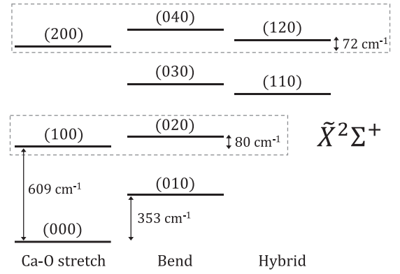
FIG. 8. Low-lying vibrational levels of the \tilde{X}^2\Sigma^+ state of CaOH. Groups of near-degenerate states with significant Fermi resonance mixing considered in this work are indicated by gray boxes. Note that Fermi resonance between (11 10 ) and (03 10 ) may also occur but is not considered here.
