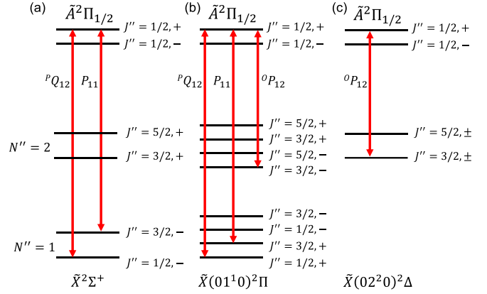
FIG. 2. Allowed rotational transitions for \tilde{A}^2\Pi_{1/2} \leftarrow \tilde{X}^2\Sigma^+ CaOH laser cooling. (a) All nondegenerate ground states of {}^2\Sigma^+ symmetry [e.g., (000), (100), (02 0 0)] have only two allowed rotational components split by \sim 50 MHz. Hyperfine splittings of 1.5 MHz and 7 kHz in the J'' = \frac{3}{2} and J'' = \frac{1}{2} states, respectively [28], are not shown. (b) Because of parity doubling in states of {}^2\Pi symmetry [e.g., (01 1 0)], additional decay is allowed to the N'' = 2 rotational level. This must be repumped using an additional laser frequency \sim 40 GHz away from the N'' = 1 transition. (c) States with {}^2\Delta symmetry [e.g., (02 2 0), (12 2 0)] have no N'' = 1 component, so only the {}^O P_{12} line must be addressed. Note that decay from \tilde{A}^2\Pi_{1/2}(000) to the \ell \neq 0 states in (b) and (c) is symmetry forbidden, and only occurs due to vibronic perturbations in the excited state (Sec. III).
