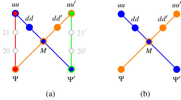
FIG. 6. Hypergraphs of the “orthogonality backbones” of (a) Fig. 5(a) and (b) Fig. 5(b) supporting the two-valued states depicted in Figs. 5(c) and 5(d), respectively.
