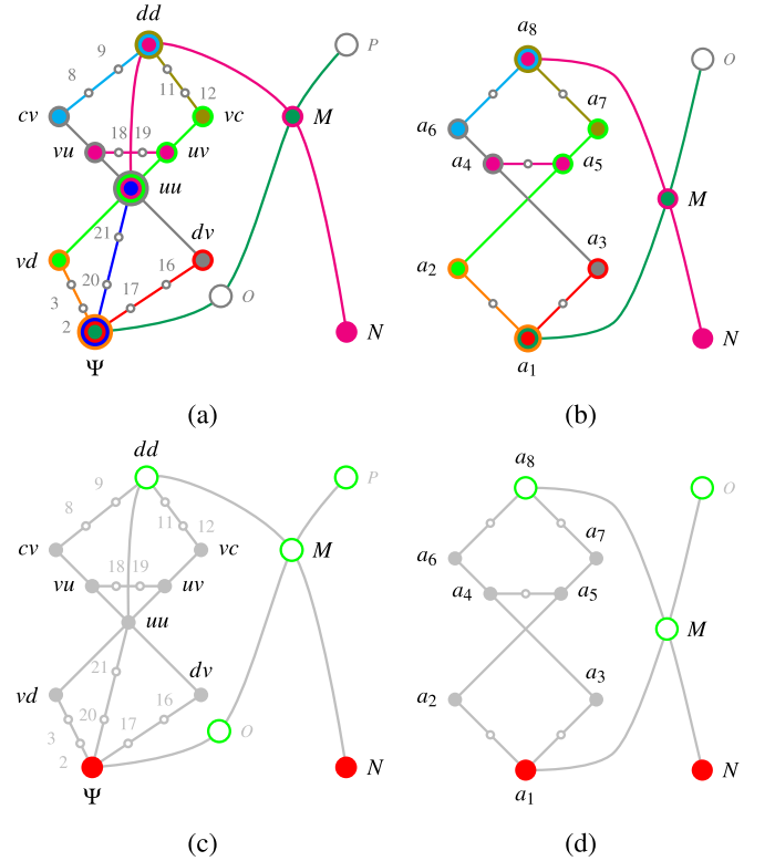
FIG. 4. Orthogonality hypergraphs of (a) the Hardy gadget extended to a true-implies-true gadget [14], as enumerated in (c), with 8 + 2 = 10 contexts and 21 + 4 = 25 atoms \{\{dd, 8, 9, cv\}, \{dd, 11, 12, vc\}, \{cv, vu, uu, dv\}, \{vc, uv, uu, vd\}, \{vu, 18, 19, uv\}, \{vd, 2, 3, \Psi\}, \{uu, 20, 21, \Psi\}, \{dv, 16, 17, \Psi\}, \{5, dd, M, N\}, \{1, O, P, M\}\} ; (b) rendition based on the true-implies-true extended Specker bug or cat’s cradle gadget [7,8], as enumerated in (c), with 7 + 2 = 9 contexts and 13 + 3 = 17 atoms \{\{a_8, \dots, a_6\}, \{a_8, \dots, a_7\}, \{a_6, a_4, a_3\}, \{a_7, a_5, a_2\}, \{a_4, \dots, a_5\}, \{a_2, \dots, a_1\}, \{a_3, \dots, a_1\}, \{a_8, M, N\}, \{a_1, \dots, M\}\} . Due to the way these true-implies-false gadgets are constructed, N always turns out to be 1 if \Psi or a_1 are supposed to be 1. Small circles indicate “auxiliary” observables, which can be chosen freely, subject to orthogonality constraints: all smooth lines indicate respective contexts representing orthonormal bases.
