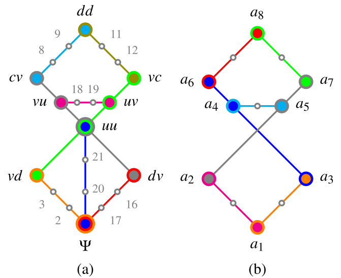
FIG. 1. Orthogonality hypergraphs of (a) the Hardy gadget with 8 contexts and 21 atoms \{\{dd, 8, 9, cv\}, \{dd, 11, 12, vc\}, \{cv, vu, uu, dv\}, \{vc, uv, uu, vd\}, \{vu, 18, 19, uv\}, \{vd, 2, 3, \Psi\}, \{uu, 20, 21, \Psi\}, \{dv, 16, 17, \Psi\}\} ; (b) rendition of the true-implies-false Specker bug gadget with 7 contexts and 13 atoms \{\{a_8, \dots, a_6\}, \{a_8, \dots, a_7\}, \{a_6, a_4, a_3\}, \{a_7, a_5, a_2\}, \{a_4, \dots, a_5\}, \{a_2, \dots, a_1\}, \{a_3, \dots, a_1\}\} . Small circles indicate “auxiliary” observables which can be chosen freely, subject to orthogonality constraints: all smooth lines indicate respective contexts representing orthonormal bases. Larger circles indicate observables common to two or more intertwining contexts.
