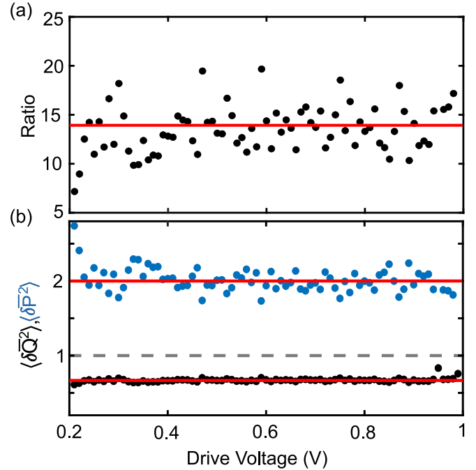
FIG. 7. (a) Ratio of the areas of the satellites peaks obtained from the quadrature data as a function of the drive voltage (black dots). The red solid line corresponds to the theoretical prediction (13). (b) Normalized dimensionless variances of the in-phase and quadrature fluctuations \langle \delta Q^2 \rangle = (\omega_0^2/k_B T) \langle \delta Q^2 \rangle and \langle \delta P^2 \rangle = (\omega_0^2/k_B T) \langle \delta P^2 \rangle around the stable state of the forced vibration as functions of the drive voltage. Black and blue dots show the in-phase and quadrature values extracted from the experimentally determined satellite area ratio from (a), whereas the red solid lines show the corresponding theoretical model of Eq. (14). The gray dashed line illustrates the thermomechanical fluctuations at the temperature 293 K used in the experiment.
