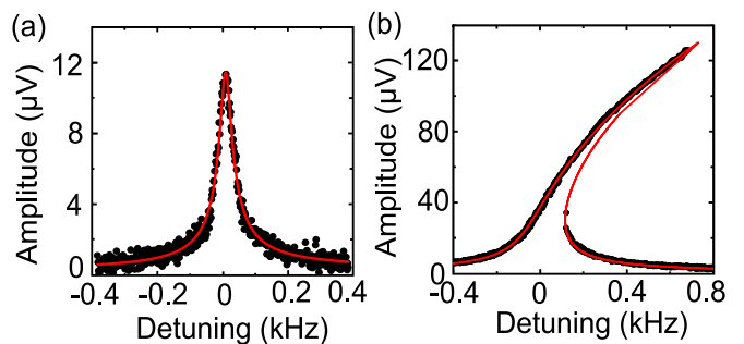
FIG. 5. (a) Linear response of the fundamental flexural out-of-plane mode at a drive voltage of V_d = 3 mV (black dots). A Lorentzian fit (red solid line) yields an eigenfrequency of 6.562 MHz, a linewidth of 2\Gamma/2\pi = 35 Hz, and a quality factor Q \approx 190\,000 . (b) Duffing response at a drive voltage of V_d = 35 mV (black dots) and fit with the Duffing model (red solid line). The resulting Duffing nonlinearity is \gamma/(2\pi)^2 = 7.6 \times 10^{17} \text{ V}^{-2} \text{ s}^{-2} .
