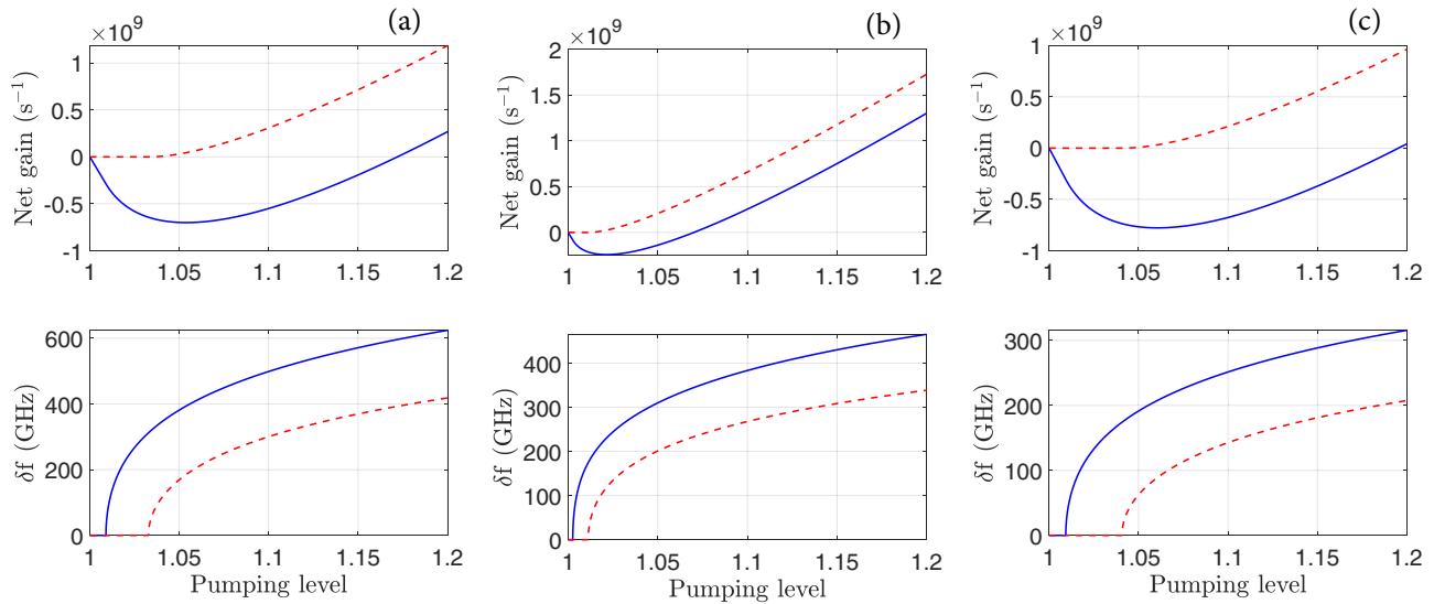
FIG. 9. Dependence of the gain peak for side modes on the pumping level for different relaxation times: (a) T_1 = 0.5 ps and T_2 = 0.05 ps, (b) T_1 = 1.0 ps and T_2 = 0.05 ps, and (c) T_1 = 1.0 ps and T_2 = 0.10 ps. In each subfigure, the upper panel shows the gain value at the peak and the lower panel shows the frequency detuning \delta f of the gain peak from the central lasing mode. Blue solid line is for \phi = 0 and red dashed line is for \phi = \pi .
