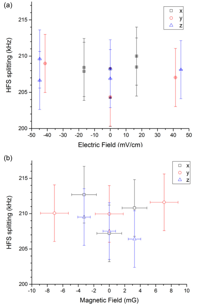
FIG. 3. Measured HFS splitting as the electric (a) and magnetic (b) fields are changed one direction at a time, with all other field components compensated to zero (within our uncertainties). All data were obtained for the 45P_{3/2} \rightarrow 45S_{1/2} microwave transition. Vertical error bars result from adding in quadrature the 1\sigma uncertainties in the individual line centers. Horizontal error bars reflect voltage and current uncertainties for (a) and (b), respectively. Horizontal error bars in (a) are not visible because of their small value ( \leq 0.2 mV/cm).
