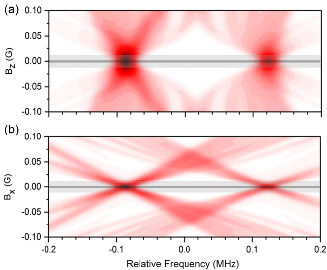
FIG. 4. Calculations of the 45P_{3/2} \rightarrow 45S_{1/2} F'' = 3 (left peak) and F'' = 2 (right peak) hyperfine peaks as a function of a parallel (a) and a transverse (b) magnetic field. Highest final-state population is shown in dark red, while white is zero. The dark gray horizontal bar shows the uncertainty in our magnetic-field zeroing (2.5 mG), while the light gray horizontal bar shows the range of magnetic fields applied to obtain the data in Fig. 3(b).
