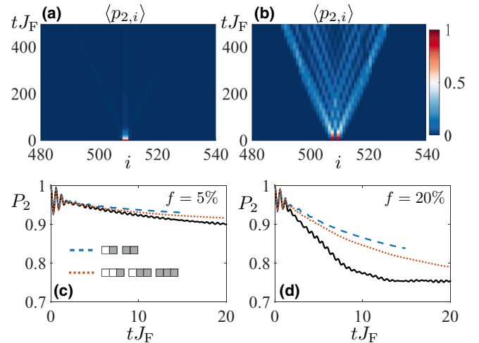
FIG. 3. (a),(b) Long-time evolution of the doublon density in a 1D lattice ( L = 1010 ) with two initial doublons computed using t-DMRG. Parameters are J_{\text{B}} = 0.1J_{\text{F}} , U_{\text{BB}} = J_{\text{F}} , and U_{\text{BF}} = 10J_{\text{F}} . In (a) the initial doublons are located on neighboring sites, and there is a fast decay on a time scale of t \sim J_{\text{B}}^{-1} = 10J_{\text{F}}^{-1} . In (b) the initial doublons are separated by an empty site. Here, the doublons are long-lived and diffuse on a time scale of t \sim J_{\text{D}}^{-1} = 100J_{\text{F}}^{-1} . In this case the doublons do not decay by forming a triplon and singlon due to the quantum Zeno effect (see text). (c),(d) Time evolution of a system with L = 100 sites and a random distribution of initial doublons with different filling fractions of f = 5\% and f = 20\% [panels (c) and (d), respectively]. For low fillings and short times, the exact t-DMRG solution (solid black line, average over 30 initial configurations) is well reproduced by considering dynamics of small connected clusters. The dashed blue (dotted red) line shows weighted averages of evolution of connected clusters with two (three) doublons, respectively.
