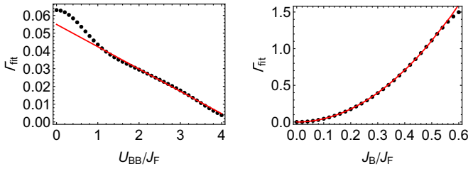
FIG. 5. Doublon decay in 2D. Fitted decay rate \Gamma from fitting P_2(t) with \exp[-\Gamma t] as a function of U_{\text{BB}}/J_F at J_B/J_F = 0.1 (left) and of J_B/J_F at U_{\text{BB}}/J_F = 1 (right). Solid lines are a linear fit to the region 1 < U_{\text{BB}}/J_F < 2d , and a quadratic fit, respectively. A lattice of size 22 by 23 sites was used with the doublon pair initially sitting on the two central sites.
