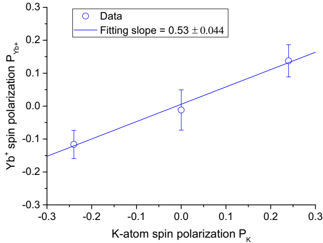
FIG. 4. Measured steady-state spin polarization of Yb + ions versus K-atom spin polarization. The fitting line is with 95% confidence level and its slope allows us to determine the spin-exchange rate coefficient.
