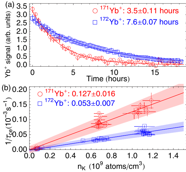
FIG. 2. (a) Decay signals of Yb + ions due to ion loss under the presence of \sim 7 \times 10^8 \text{ cm}^{-3} K-atom number density. The data are fitted to an exponential function to extract \tau_{ce} . The numbers represent the charge-exchange time constants and the fitting errors. (b) The charge-exchange rate of a Yb + ion under different potassium densities. Experimental data of 171 Yb + ( 172 Yb + ) ions are shown in red circles (blue squares). The data are fitted to a linear function to extract the slope and to determine the upper bound of \kappa_{ce} . The shaded areas represent 95% confidence interval.
