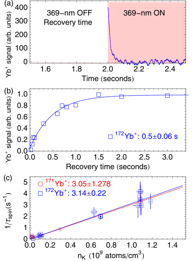
FIG. 3. (a) Red shaded area represents the 50-nW, 0.5-s pulse of the circularly polarized 369-nm laser light. (b) The data points with a normalized scale represent the areas under of the fluorescence transient curves for different recovery time periods, where n_{\text{K}} \sim 7 \times 10^8 \text{ cm}^{-3} . The numbers represent the spin recovery time constants and the fitting errors. Each data point is an average of 200 runs. (c) The spin recovery time constants versus different K number densities. Data of ^{172}\text{Yb}^+ ions and ^{171}\text{Yb}^+ ions are shown in blue square markers and red circle markers, respectively. The ^{171}\text{Yb}^+ data uses similar procedure for ^{172}\text{Yb}^+ except that the 369-nm laser is linearly polarized at 5 \mu\text{W} with 3.5-s pulse width. The solid lines represent the linear fitting results. The fitting lines are with 95% confidence level.
