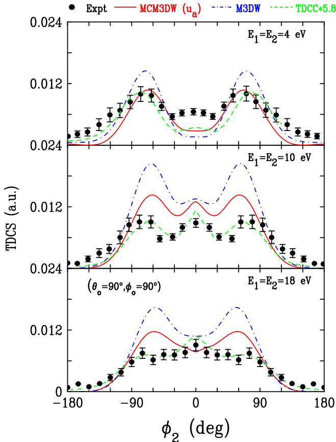
FIG. 5. Comparison of experimental and theoretical TDCS for electron-impact ionization of orientated H_2 with the ejected electron being detected in the perpendicular plane at angle \phi_2 . Both final-state electrons have equal energies as indicated. The experimental data are those of Ren et al. [22] and the H_2^+ ion is orientated at (\theta_0 = 90^\circ, \phi_0 = 90^\circ) . The theoretical calculations are the MCM3DW ( u_a ) (solid red curve), the M3DW (dashed-dot blue curve), and the TDCC (dashed green). The normalization factor is the same as that used in Fig. 2.
