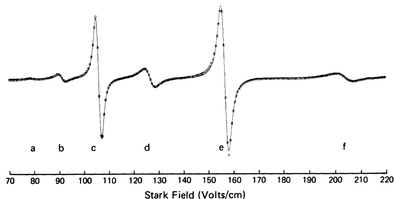
FIG. 1. Optical-double-resonance spectrum for ^{13}\text{CH}_3\text{F} at \sim 3 mTorr pressure and \Omega_1 - \Omega_2 = 30.008 MHz. The optical selection rule is \Delta M = \pm 1 . Lines c and e correspond to the level configuration of Fig. 2(a) and the others to Fig. 2(b). The Stark sweep is computer driven in steps and the output signal is digitized (squares) and least-squares fitted to Lorentzian line shapes (solid line). The Stark-gap spacing is 0.60256 cm and the sample path length is 10 cm (from Brewer et al. , Ref. 3).
