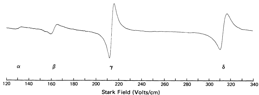
FIG. 4. Optical double-resonance spectrum for ^{13}\text{CH}_3\text{F} with \Omega_1 - \Omega_2 = 29.930 MHz. The optical selection rule is \Delta M=0 for one transition and \Delta M=\pm 1 for the other. The spectrum is displayed directly on an x-y recorder as the Stark field is swept continuously. The phase of the detector is reversed by \pi from Fig. 1. Lines \gamma and \delta correspond to the level structure of Fig. 2(a) and \alpha and \beta to Fig. 2(b). Line \rho of Table IV is not displayed here.
