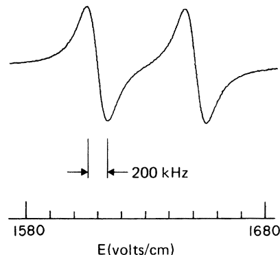
FIG. 5. Optical-double-resonance spectrum for ^{12}\text{CH}_3\text{F} with \Omega_1 - \Omega_2 = 39.629 MHz. The optical selection rule is \Delta M = \pm 1 . (See Ref. 8 for details.) The lines correspond to the level structure of Fig. 2(a).
