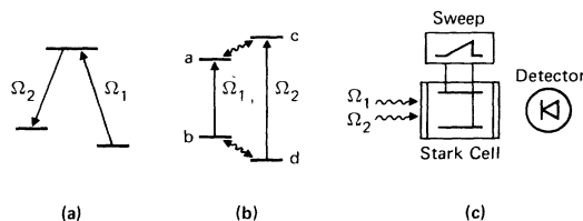
FIG. 2. (a) Traditional double-resonance level configuration; (b) collision-induced double-resonance level configuration, with wavy lines indicating collision-induced transitions; (c) experimental arrangement for monitoring optical double-resonance signals.
