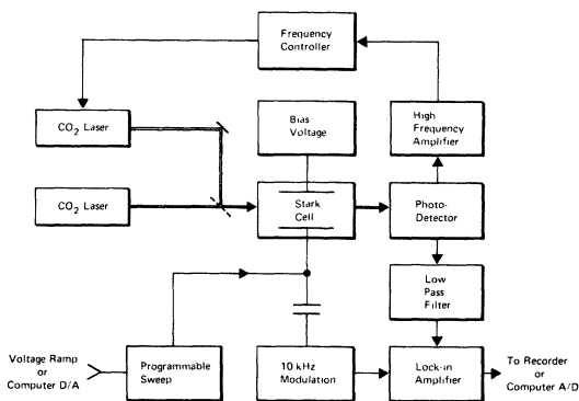
FIG. 3. Block diagram of the double-resonance experiment.
