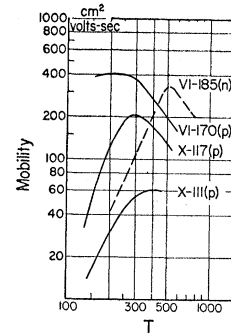
FIG. 4. Charge carrier mobilities of GaSb.
