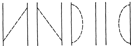
FIG. 1. Three-dimensional Feynman diagrams contributing to the second-order interaction of two nucleons.
