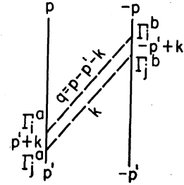
FIG. 4. Labels used in writing the matrix element [Eq. (III.1)] for diagram (1a) of Fig. 3.
