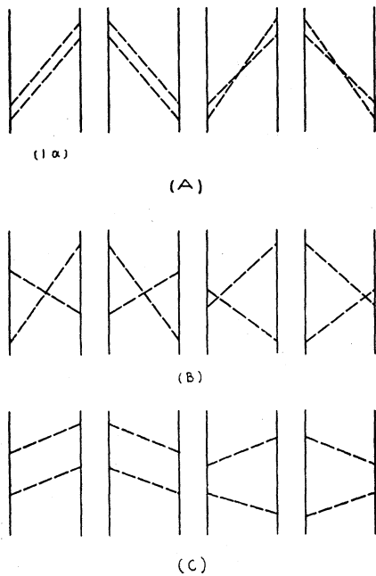
FIG. 3. The set (A) of fourth order diagrams contain the main spurious divergences in Dyson's new Tamm-Dancoff method. The sets (B) and (C) do not contain terms proportional to (2M)^{-2} . Because of the time ordering of the interaction, all the diagrams in the Tamm-Dancoff method can be divided into pairs. Of the above 12 interaction terms one need only calculate the 6 corresponding matrix elements. The remaining six can be obtained by a reflection of time. As an example, we give in Eq. (III.1) the matrix element that corresponds to the diagram labeled (1a).
