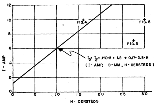
FIG. 1. Minimum current as function of the longitudinal magnetic field H for the Sn-sample used by Mendelsohn et al.
