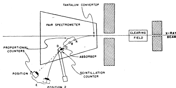
FIG. 1. Experimental arrangement.
