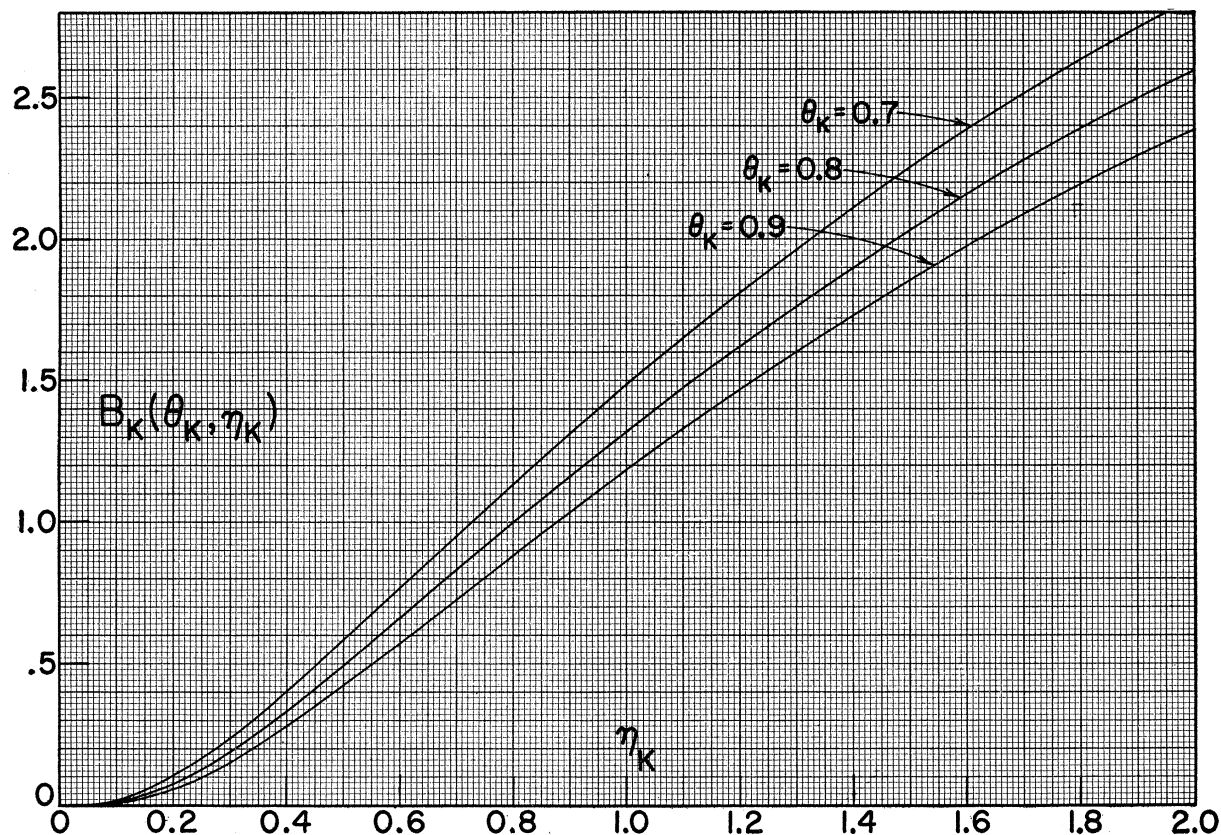
FIG. 1. B_K(\theta_K, \eta_K) , stopping number contribution of ^1_2K -electrons.
