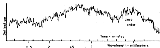
FIG. 2. Solar spectrum obtained with an echelette grating.
