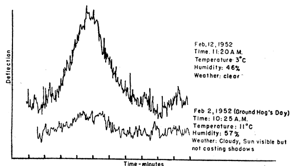
FIG. 1. Transits of the sun across the field of the millimeter wave telescope.
