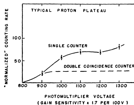
FIG. 3. Plateau for counting high energy protons. — line is for a single counter, - - - line is for two counters in coincidence.
