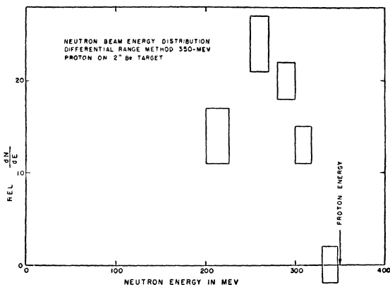
FIG. 2. Energy distribution of neutron beam produced by 340-Mev protons bombarding a \frac{1}{2} -in. beryllium target.
