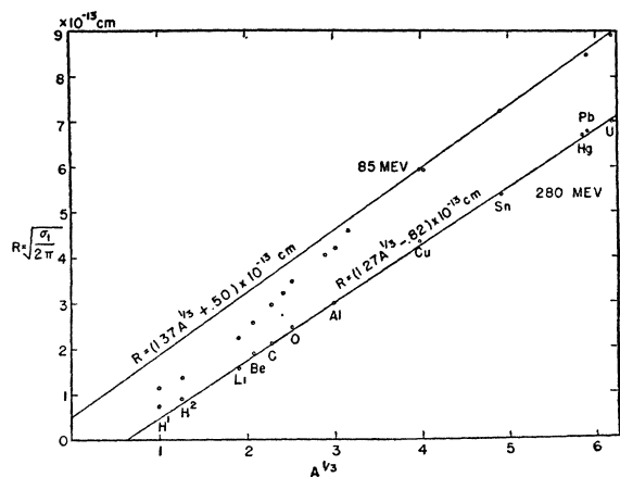
FIG. 4. "Effective radius" R = (\sigma_t/2\pi)^{1/2} plotted against A^{1/3} . 85-Mev results shown also for comparison.
