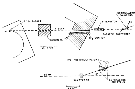
FIG. 1. Experimental arrangement for measurement of total cross sections. For measurement of neutron beam energy distribution, the scatterer is alternately carbon and paraffin, the copper absorber thickness is varied, and there is no attenuator.
