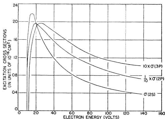
FIG. 6. Electronic excitation cross sections for states of atomic hydrogen calculated by Born approximation without exchange.
