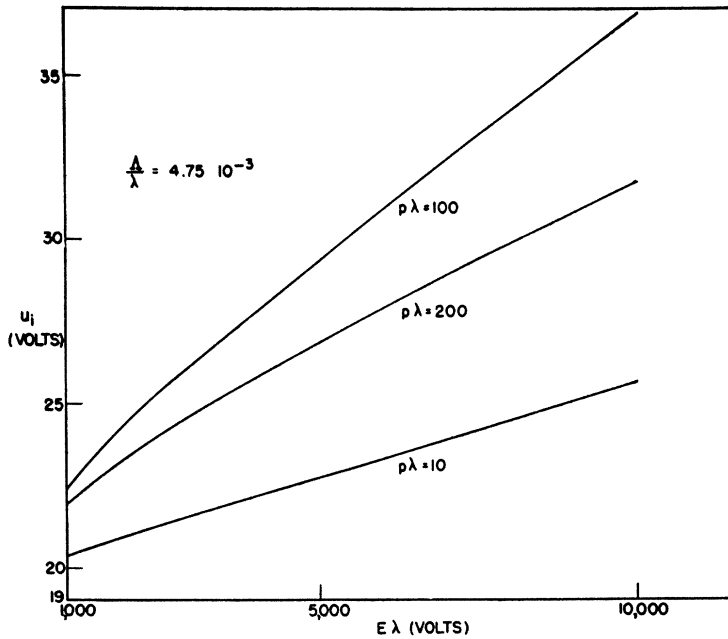
FIG. 4. The effective ionization potential as a function of E\lambda at a constant \Delta/\lambda .
