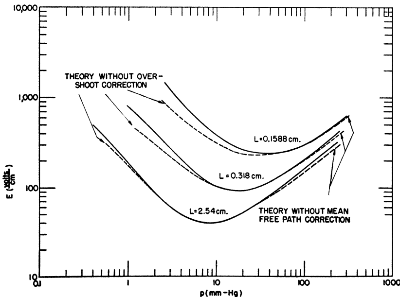
FIG. 3. Theoretical E-p curves illustrating the effect of the correction factors of Sections VI and VII. The broken lines indicate theoretical fields without corrections. The \frac{1}{2} -inch cavity is omitted to avoid confusing the diagram.
