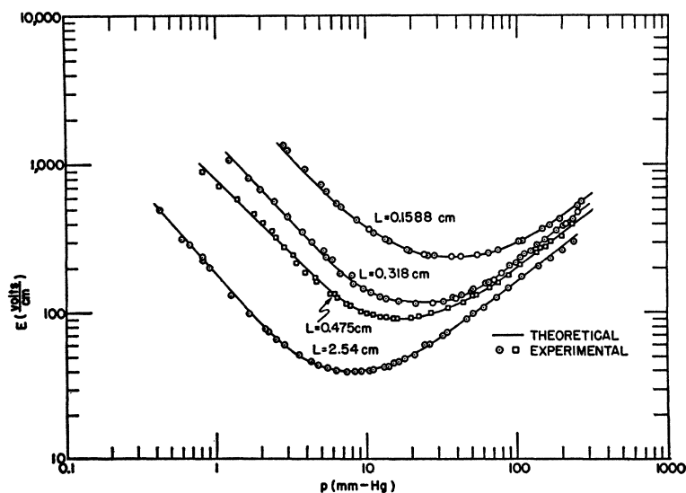
FIG. 6. Experimental breakdown electric fields compared with those theoretically predicted.
