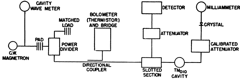
FIG. 5. Block diagram of the experimental microwave equipment.
