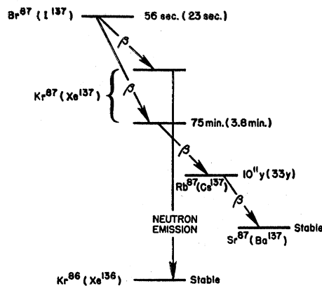
FIG. 2. Possible branching mechanism which would account for the low yield of the bromine and iodine delayed neutrons in comparison with the yields of fission products of mass 87 and 137. It is presumed that only a small proportion of the atoms choose the low energy beta-transition which is followed by neutron emission.
