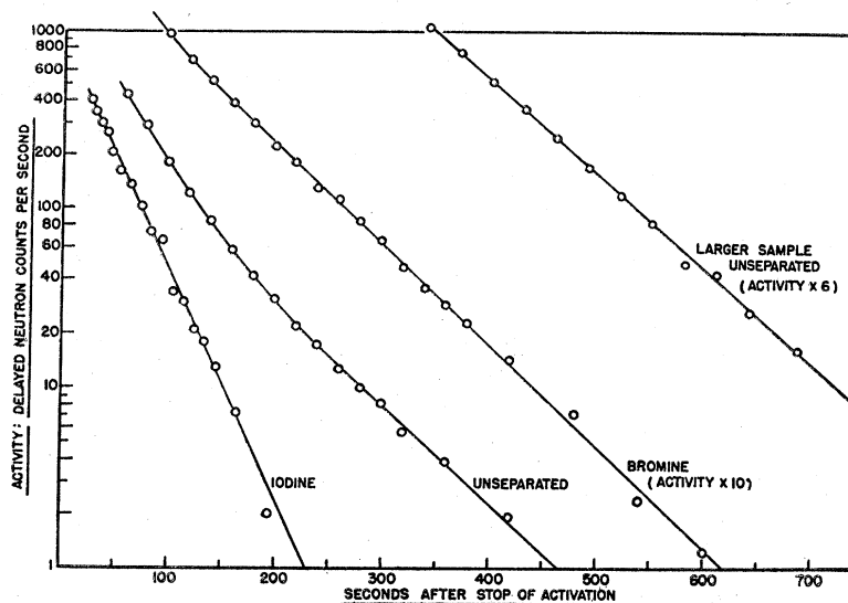
FIG. 1. Decay curves of the delayed neutrons emitted from uranium ("unseparated") and from the separated iodine and bromine fission products. The decay of the longest period in the unseparated sample is seen to be parallel to that of the bromine fraction. The relative intensities between the various curves are to be disregarded.
