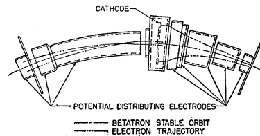
FIG. 1. Schematic drawing of on-orbit injector. The magnetic field is normal to the paper.
