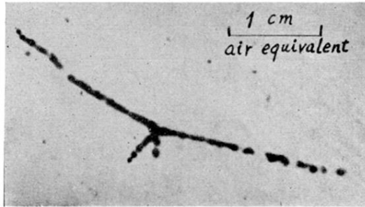
FIG. 4. Quaternary fission.
