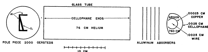
FIG. 1. Experimental arrangement.
